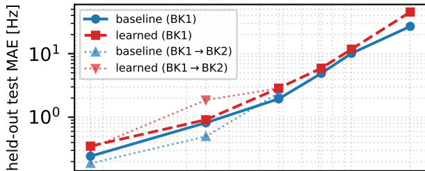
(a) learned never beats baseline
