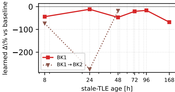
(b) relative degradation (all < 0)
