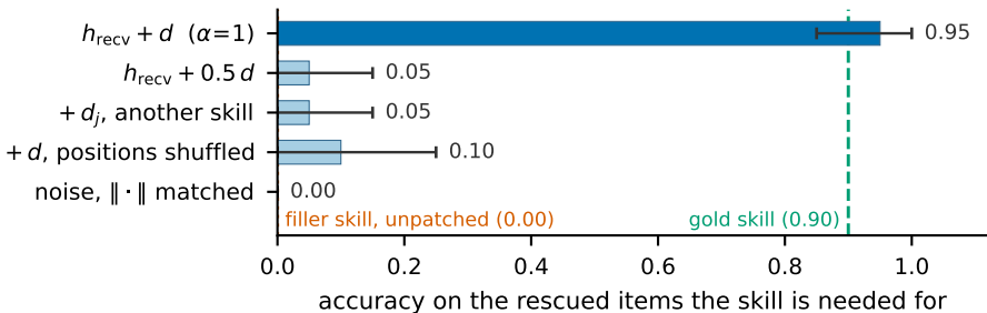
written over the skill's own span ( n = 20 )
