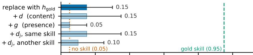
written at the last prompt position ( n = 20 )
