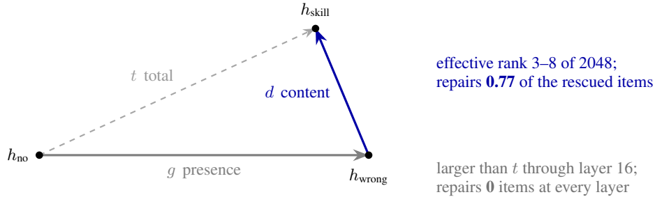
Figure 7: The decomposition, drawn to scale at layer 10 of the synthetic control ( \|g\| = 39.0 , \|d\| = 16.3 , \|t\| = 36.0 ). A document of the right length and the wrong content already moves the final prompt position most of the way—in fact slightly further than the real skill does, which is why the content arrow points partly back. Everything this paper is about is the short blue arrow.
