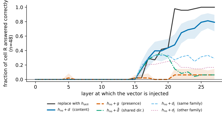
Figure 7: What each injected component repairs, on the cell the document rescues. Shaded bands are bootstrap 95% CIs for the two conditions the argument rests on. h_{no} + t is omitted because it equals h_{skill} identically and its curve lies under the black one—we run it, and it agrees item by item. Synthetic control, multiple choice, Qwen3-1.7B, fp32, n_R = 48 .
