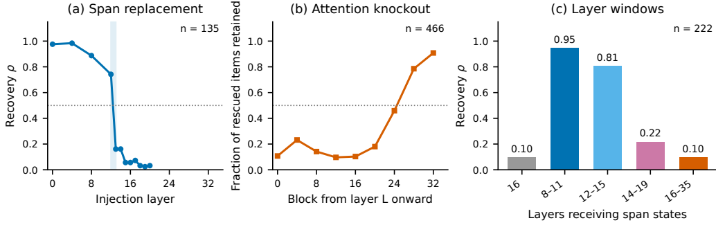
Figure 3: Transfer declines earlier than dependence on skill attention, Qwen3-8B on MedCalc. All panels use the larger rerun. (a) Single-layer span replacement on the screened subset ( n = 135 ). The shaded band marks the largest drop, between layers 12 and 13. (b) Fraction of rescued items remaining correct when attention to the skill is blocked from layer L onward ( n = 466 ). The dotted lines mark 0.5 in each panel’s own metric. (c) Repeated injection at layers 16–35 gives no gain over layer 16 alone, whereas layers 12–15 recover 0.81 ( n = 222 ). This completed window experiment uses a different wrong-content receiver and its own baselines; it is not directly paired with (a). Span interventions use the corrected implementation; attention knockout does not use state capture.
