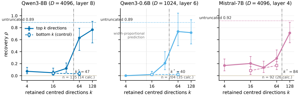
Figure 2: Recovery after retaining k leading centred directions and restoring the positional mean, on MedCalc after the fix. Each model is injected at an early layer. Despite a fourfold difference in hidden width, Qwen3-0.6B and Qwen3-8B have similar rank knees (40 and 47); Mistral-7B, with the same width as Qwen3-8B, has k^* = 84 . Untruncated recovery is 0.89, 0.89 and 0.92, respectively, on each rank experiment’s own subset. The Mistral rank subset (92 items, 26 calculators) differs from its newer battery subset in Table 4. Dashed curves retain bottom directions. Error bars are calculator-bootstrap 95% intervals. Only complete rank experiments are plotted.
