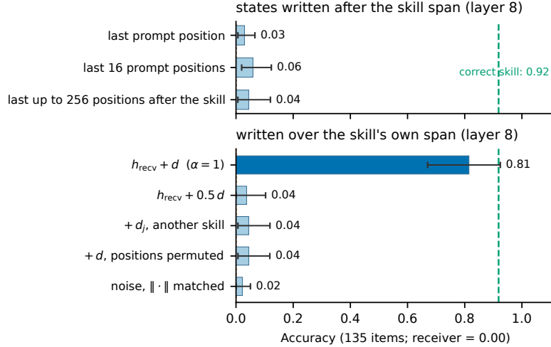
Figure 1: Matched position comparison on MedCalc with Qwen3-8B after the fix. Both panels use layer 8, the same wrong-skill receiver and 135 items from 14 calculators. Top: donor states written at the last 1, 16, or up to 256 available positions after the skill. Bottom: interventions over the skill span. The dashed line marks correct-skill accuracy; the dotted line marks receiver accuracy. Error bars are calculator-bootstrap 95% intervals.
