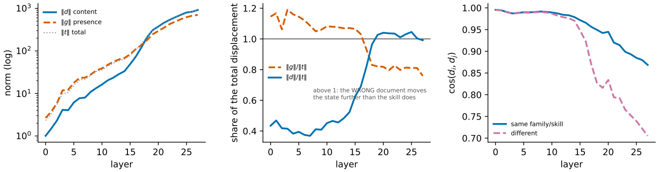
Figure 7: The decomposition across depth, synthetic control, Qwen3-1.7B, fp32, n = 358 . Left: the three norms. Middle: each component as a share of the total displacement; above 1 the wrong document moves the state further than the skill does, which is the case until layer 17. Right: how aligned two items' content vectors are, split by whether they use the same row of the conversion table.
