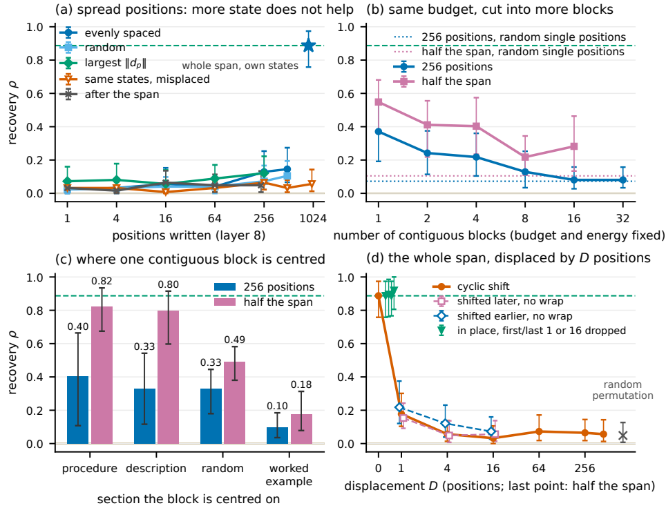
Figure 2: Position budget on MedCalc with Qwen3-8B, layer 8: the same 135 screened items (14 calculators) and wrong-skill receiver in every panel; the dashed line is the whole span written in place ( \rho = 0.89 ). (a) B positions, each written with its own donor state (evenly spaced, random, or largest \|d_p\| ), the same states written half a span away, or the last B prompt positions after the span. (b) A fixed budget written as N contiguous blocks; dotted lines are random single positions at the same budget. (c) One contiguous block centred on a section of the skill. (d) The whole span displaced by D positions, cyclically or without wrap-around; triangles write it in place without its first or last 1 or 16 positions. Error bars are calculator-bootstrap 95% intervals.
