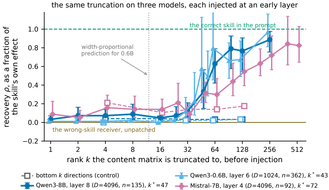
Figure 3: Recovery after retaining k leading centred directions and restoring the positional mean, on MedCalc after the fix. Each model is injected at an early layer. Despite a fourfold difference in hidden width, Qwen3-0.6B and Qwen3-8B have similar rank knees (43 and 47); Mistral-7B, with the same width as Qwen3-8B, has k^* = 72 [46, 94]. Untruncated recovery is 0.89, 0.91 and 0.84, respectively, on each model's screened subset (135, 362 and 92 items). Both Qwen models reach that value by k = 256 and Mistral-7B at k = 384 . Dashed curves retain bottom directions. Error bars are calculator-bootstrap 95% intervals. Only complete rank experiments are plotted.
