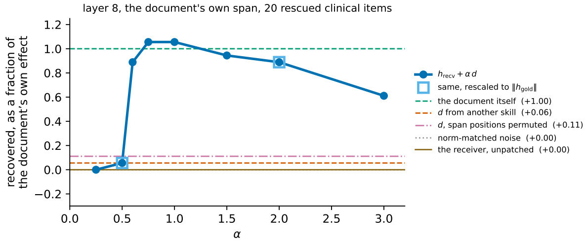
Figure 9: Dose response of the content injection over the document’s own span, layer 8, with its controls. Open squares are the same dose rescaled per position to the with-document norm; they coincide with the plain arms. Before the instrument fix; the post-fix dose sweep and norm comparison are in Appendix F.1. The horizontal lines are the three controls and the two baselines.
