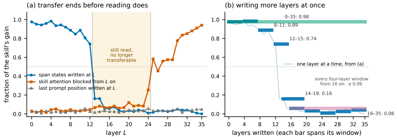
Figure 4: Transfer declines earlier than dependence on skill attention, Qwen3-8B on MedCalc, with every layer measured. (a) Three interventions on one axis and the same screened items ( n = 135 ; the knockout on their 134 rescued items): span states written at layer L ; attention to the skill blocked from L onward; and the last prompt position written at L . The shaded band spans the layers where the skill is still read but no longer transferable. (b) Each window is drawn across the layers it writes: four-layer windows tile the stack, and the long windows 14–19, 16–35 and 0–35 are shown with them; the faint curve repeats (a). Writing every layer at once recovers 0.98, while any window starting at 16 or later stays at or below 0.06. Span interventions use the corrected implementation; attention knockout does not use state capture.
