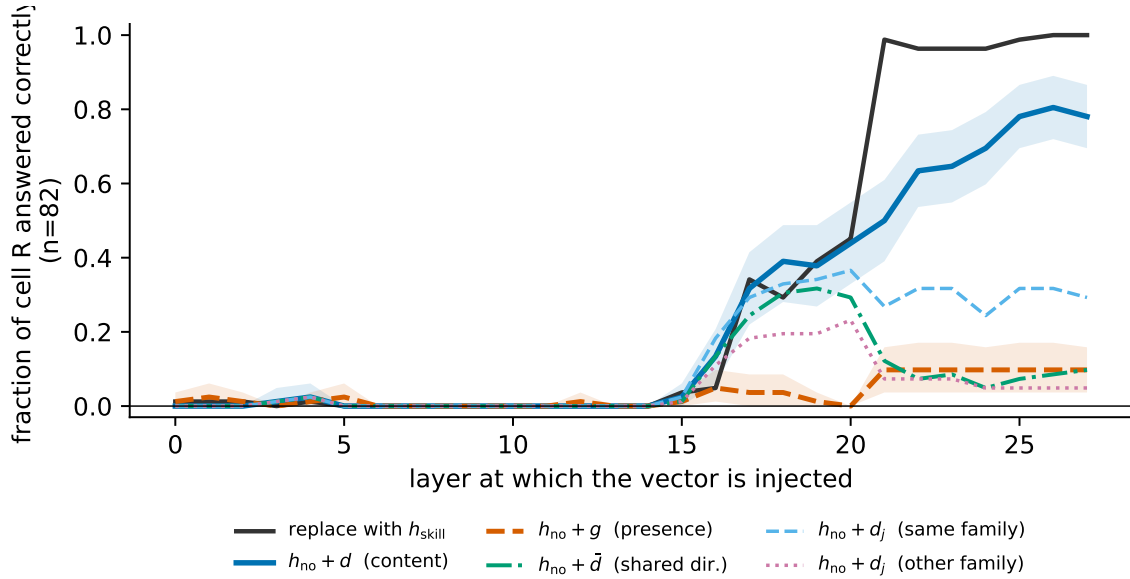
Figure 5: What each injected component repairs, on the cell the document rescues. Shaded bands are bootstrap 95% CIs for the two conditions the argument rests on. h_{no} + t is omitted because it equals h_{skill} identically and its curve lies under the black one—we run it, and it agrees item by item. Synthetic control, multiple choice, Qwen3-1.7B, fp32, n = 358 , rescued cell n_R = 82 .
