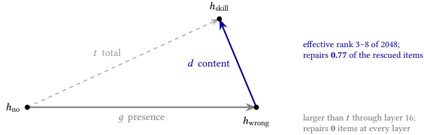
Figure 6: The decomposition, drawn to scale at layer 10 of the synthetic control ( \|g\| = 39.0 , \|d\| = 16.3 , \|t\| = 36.0 ). A document of the right length and the wrong content already moves the final prompt position most of the way—in fact slightly further than the real skill does, which is why the content arrow points partly back. Everything this paper is about is the short blue arrow.
