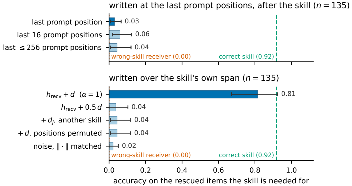
Figure 1: Matched position comparison on MedCalc with Qwen3-8B after the fix. Both panels use layer 8, the same wrong-skill receiver and 135 items from 14 calculators. Top: donor states written at the last 1, 16, or up to 256 available positions after the skill. Bottom: interventions over the skill span. The dashed line marks correct-skill accuracy; the dotted line marks receiver accuracy. Error bars are calculator-bootstrap 95% intervals.
