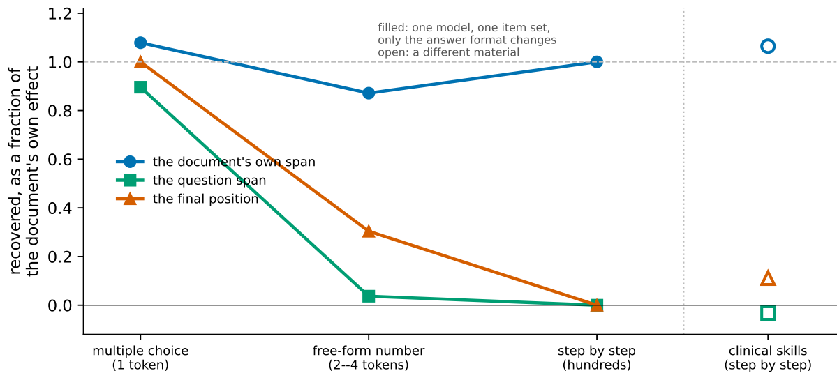
Figure 11: What each transplant channel recovers, as a fraction of what the document itself is worth in that setting, against how many tokens the answer occupies. Filled markers joined by lines are one model, one item set and one document with only the answer format changed; the clinical results are open and deliberately not joined, because that material changes the skill, the task and the prompt length at once. Plotting fractions rather than raw accuracies is necessary here: the four settings have donors at 0.550, 0.467, 1.000 and 0.950, and comparing raw numbers across them is how an earlier draft came to report that a longer answer made the document-span channel stronger. The document's own span is flat at 1.00 across every answer format. The other two channels collapse as the answer lengthens, and the clinical points land where the step-by-step column says they should.
