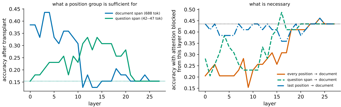
Figure 8: Left: what each position group is sufficient for, as a function of the layer at which its states are transplanted; dotted lines are each channel's own receiver baseline. Right: what is necessary—accuracy when attention to the document is masked from the given layer to the end, cumulatively; the dotted line is the unmasked baseline. Synthetic control, multiple choice, Qwen3-1.7B, n = 39 .
