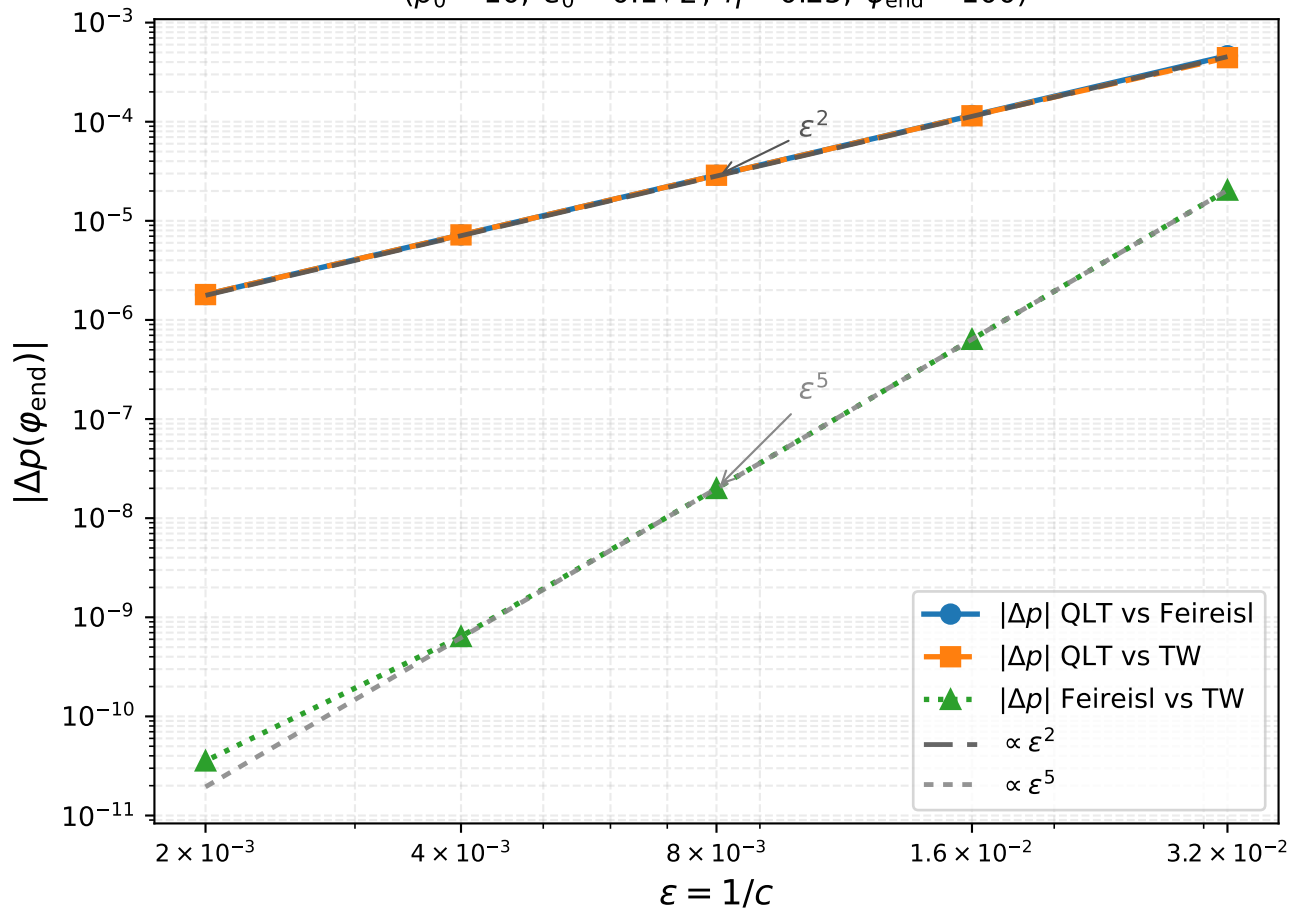
End-state convergence of p to QLT (p_0 = 10, e_0 = 0.1\sqrt{2}, \eta = 0.25, \varphi_{\text{end}} = 100)
