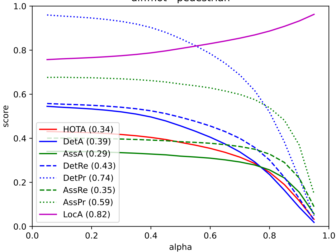
diffmot - pedestrian
