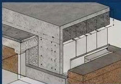
Precast Elements
