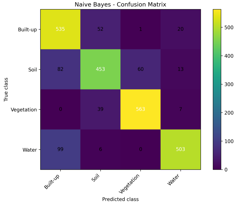
Figure 4: Confusion matrix obtained with the Gaussian Naive Bayes classifier.
