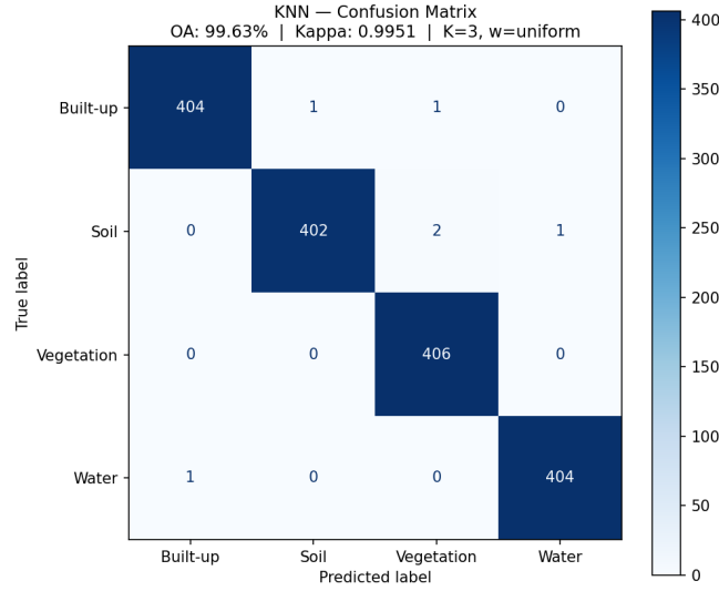
Figure 5: Confusion matrix for the KNN classifier ( K = 3 , uniform weights, Euclidean distance). OA = 99.63%, Kappa = 0.9951.
