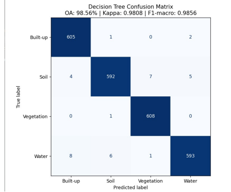
Figure 1: Confusion matrix obtained from the Decision Trees.
