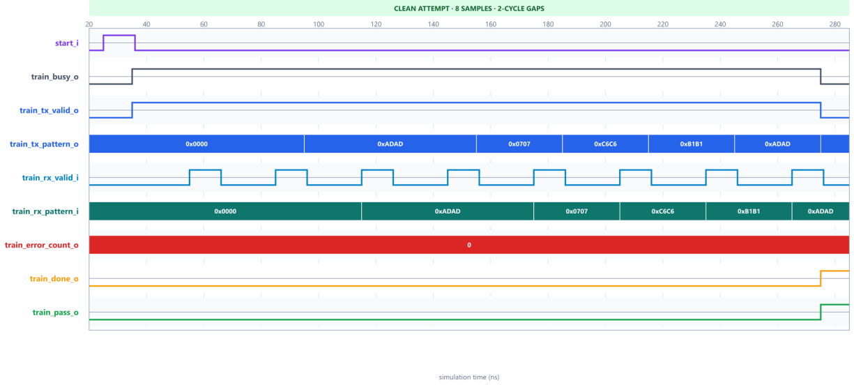
Fig. 4. Color-coded Questa waveform generated from build/waves/datatrain_lfsr.vcd . The capture shows sample-gated LFSR progression, an exact zero mismatch count, and the final done/pass decision.
