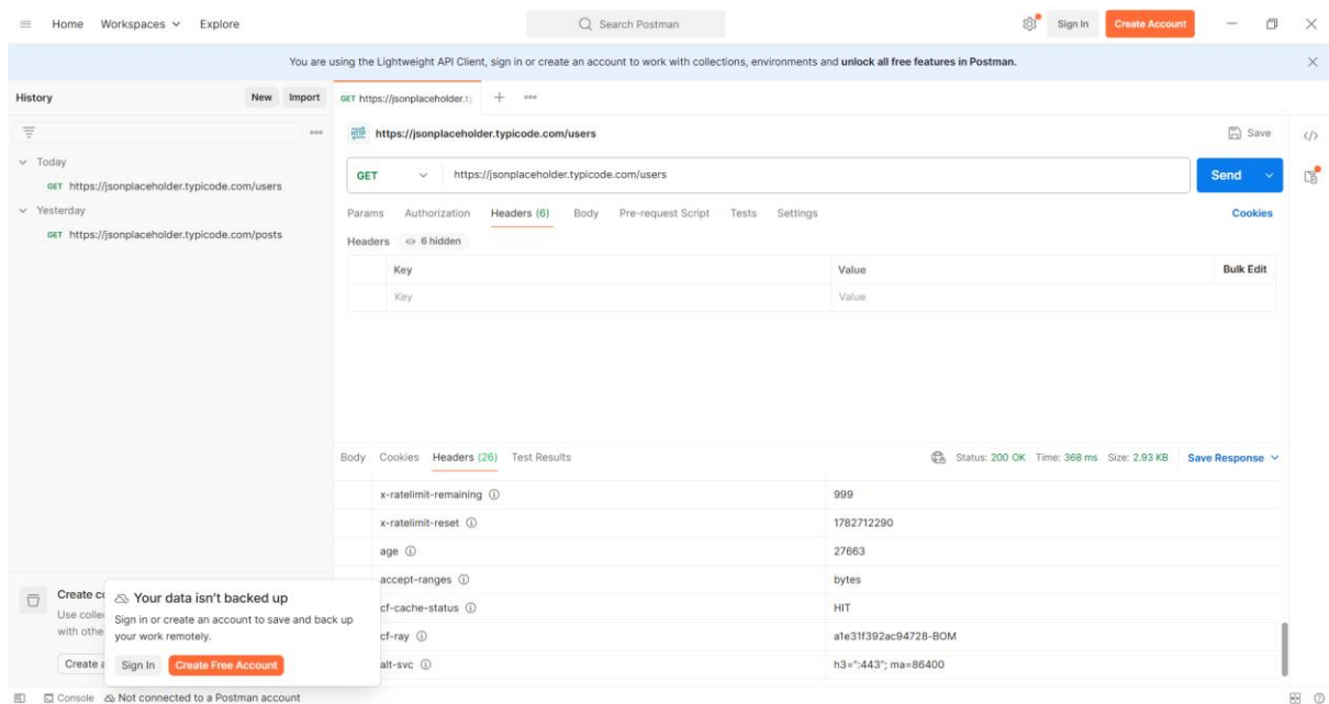
Figure 4: Response Headers
