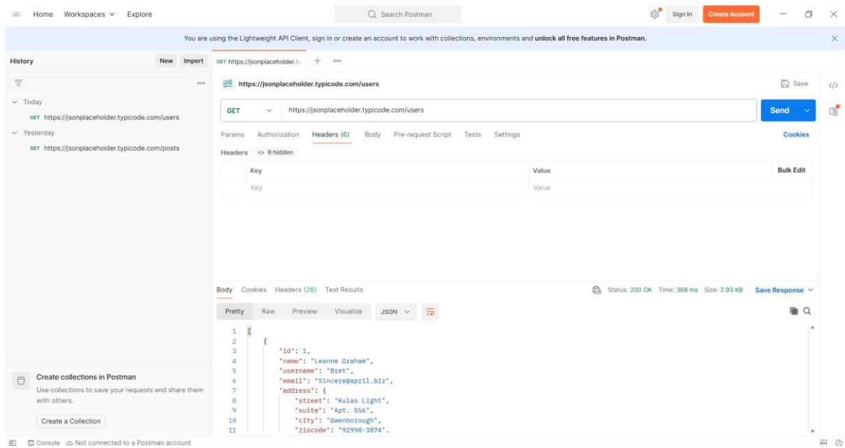
Figure 3: Request Headers
