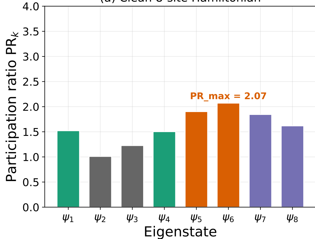
(a) Clean 8-site Hamiltonian
