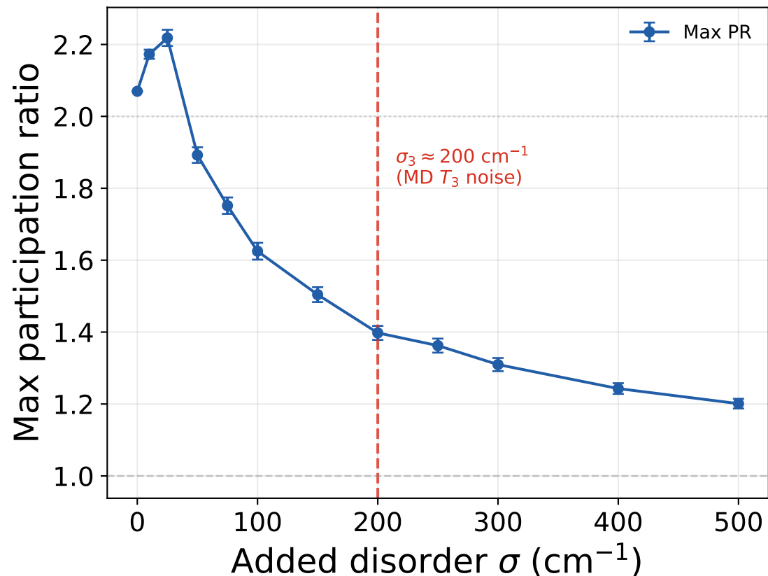
(b) Disorder scan (500 realisations)
