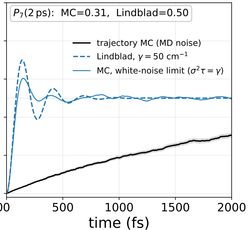
(b) MD noise vs Markovian Lindblad
