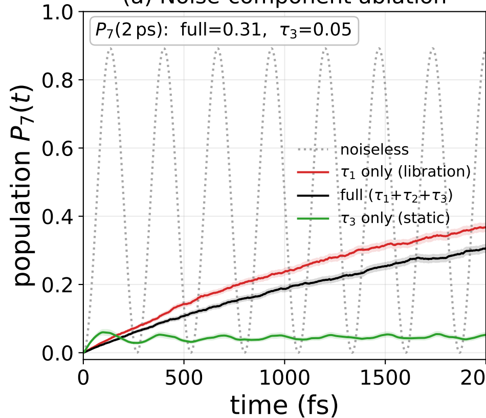
(a) Noise-component ablation
