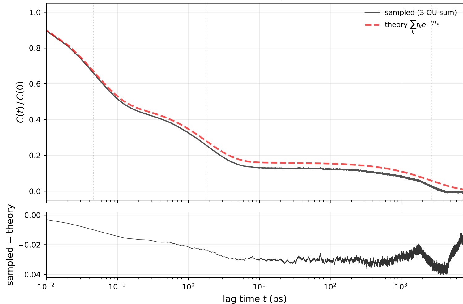
Sum of three OU processes vs analytic ACF (RMS = 0.029)
