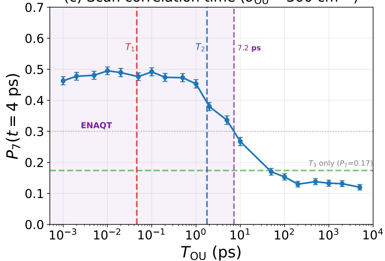
(c) Scan correlation time ( \sigma_{\text{OU}} = 300 \text{ cm}^{-1} )
