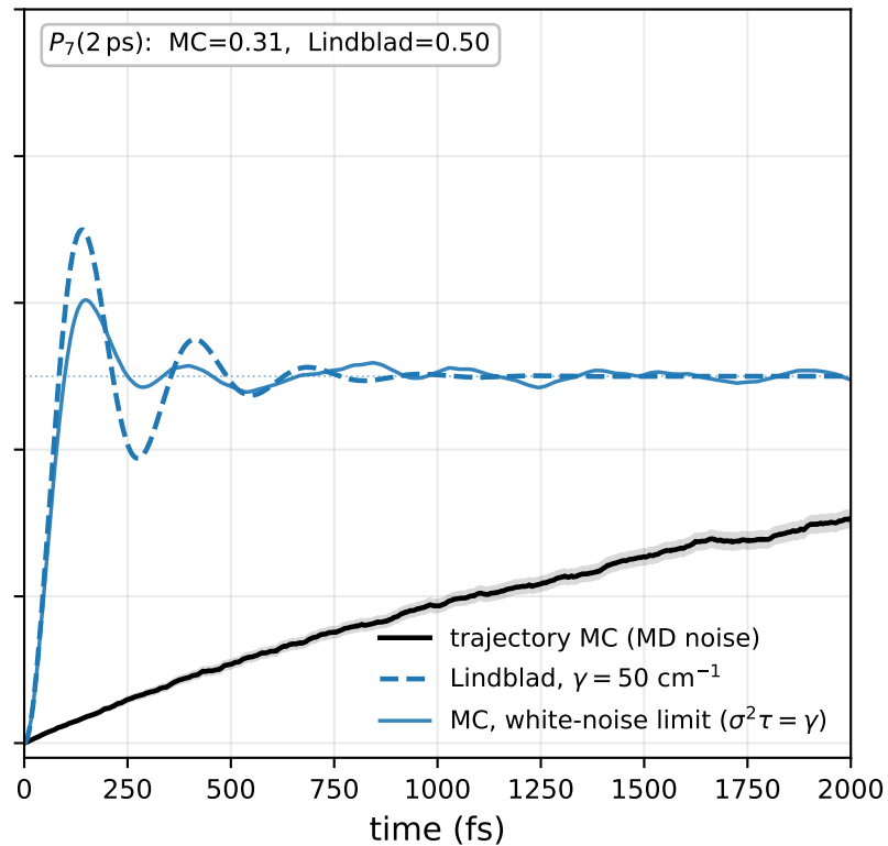
(b) MD noise vs Markovian Lindblad
