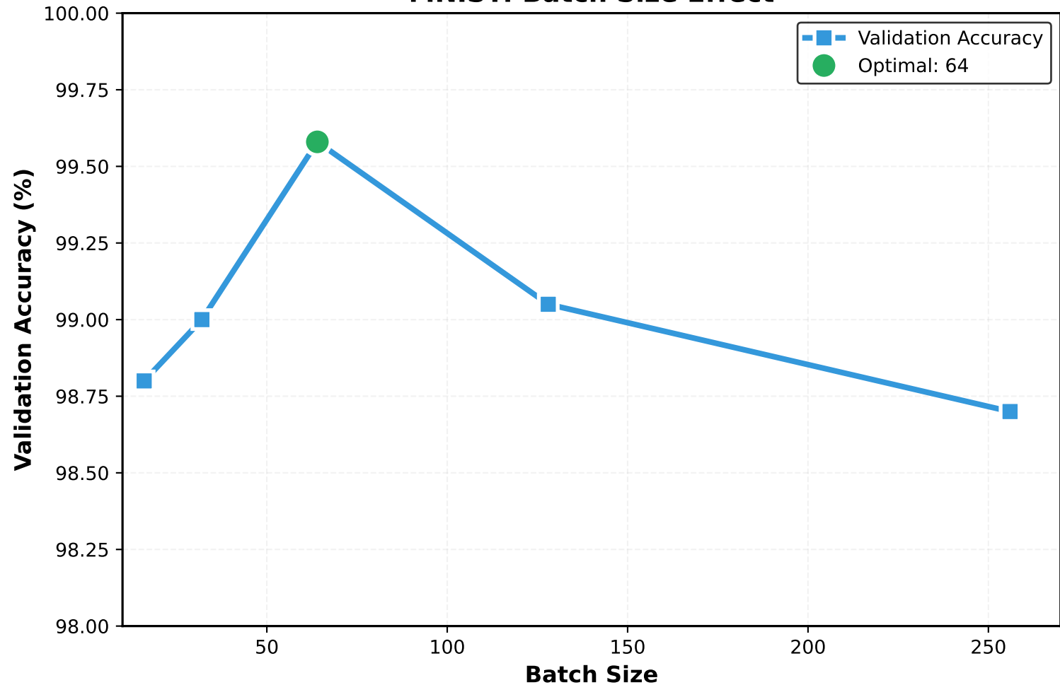
MNIST: Batch Size Effect
