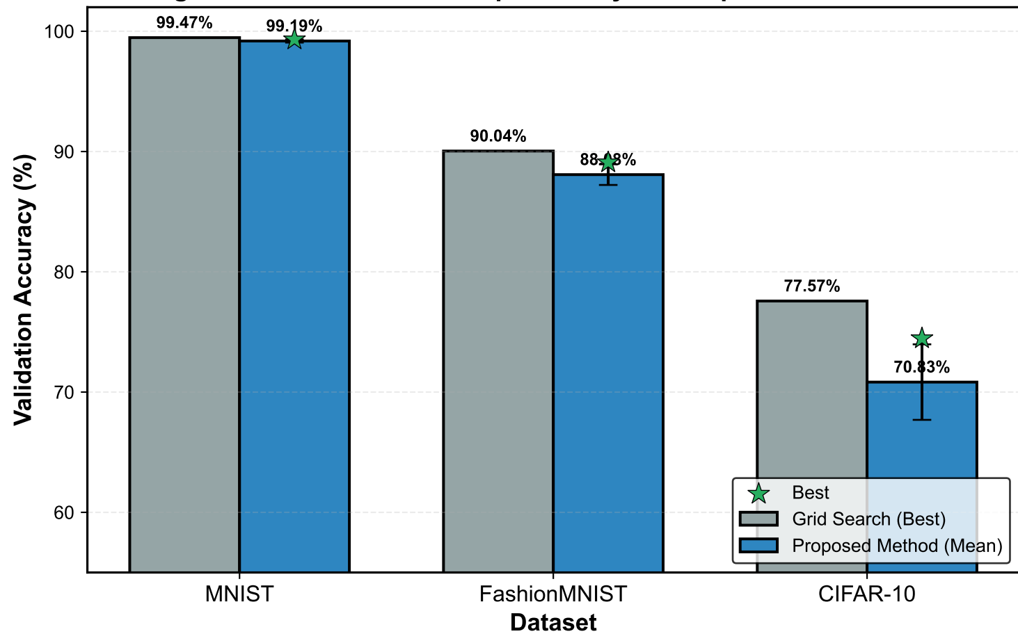
Figure 1: Final Results - Proposed Bayesian Optimization Method
