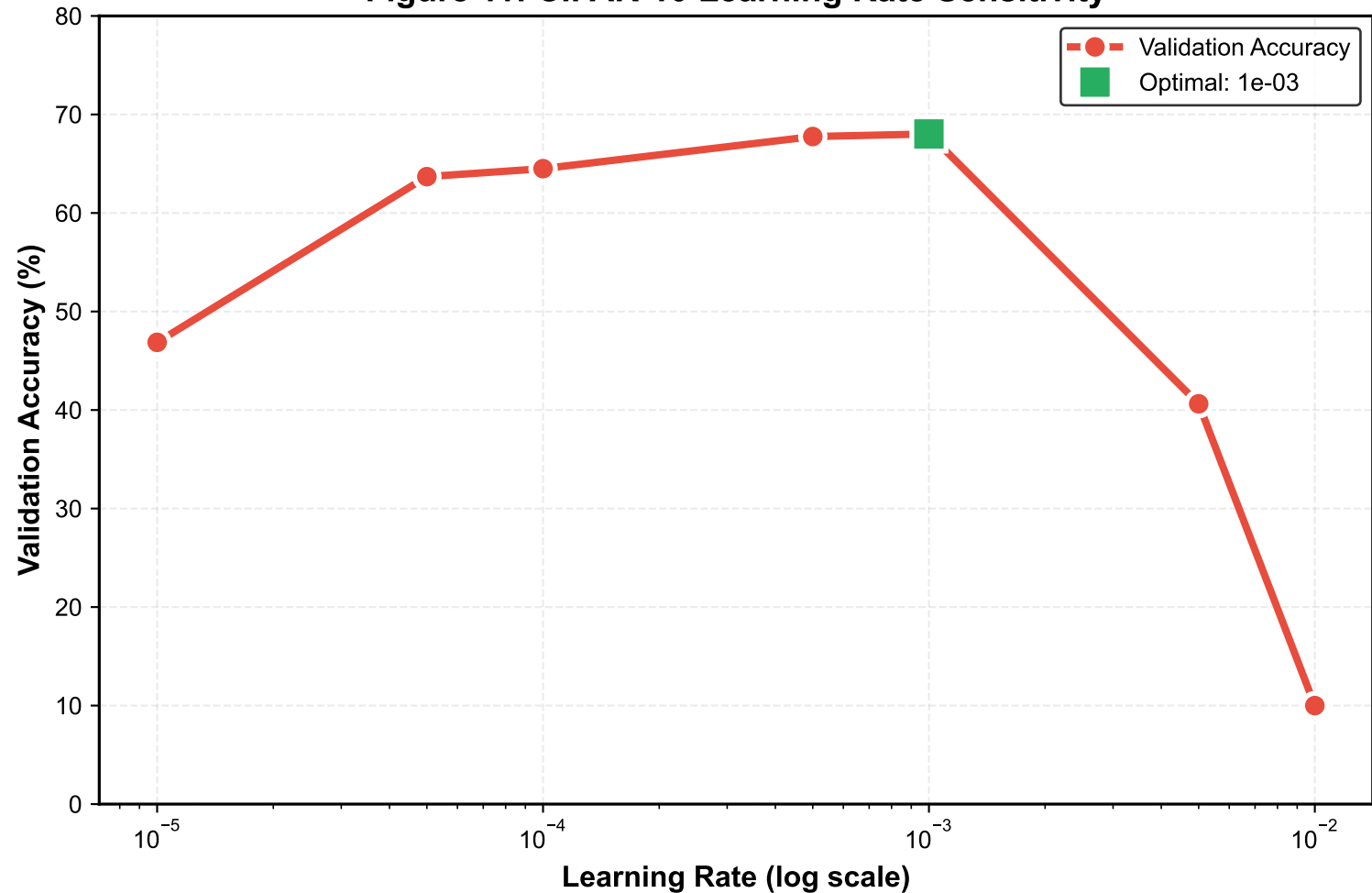
Figure 11: CIFAR-10 Learning Rate Sensitivity
