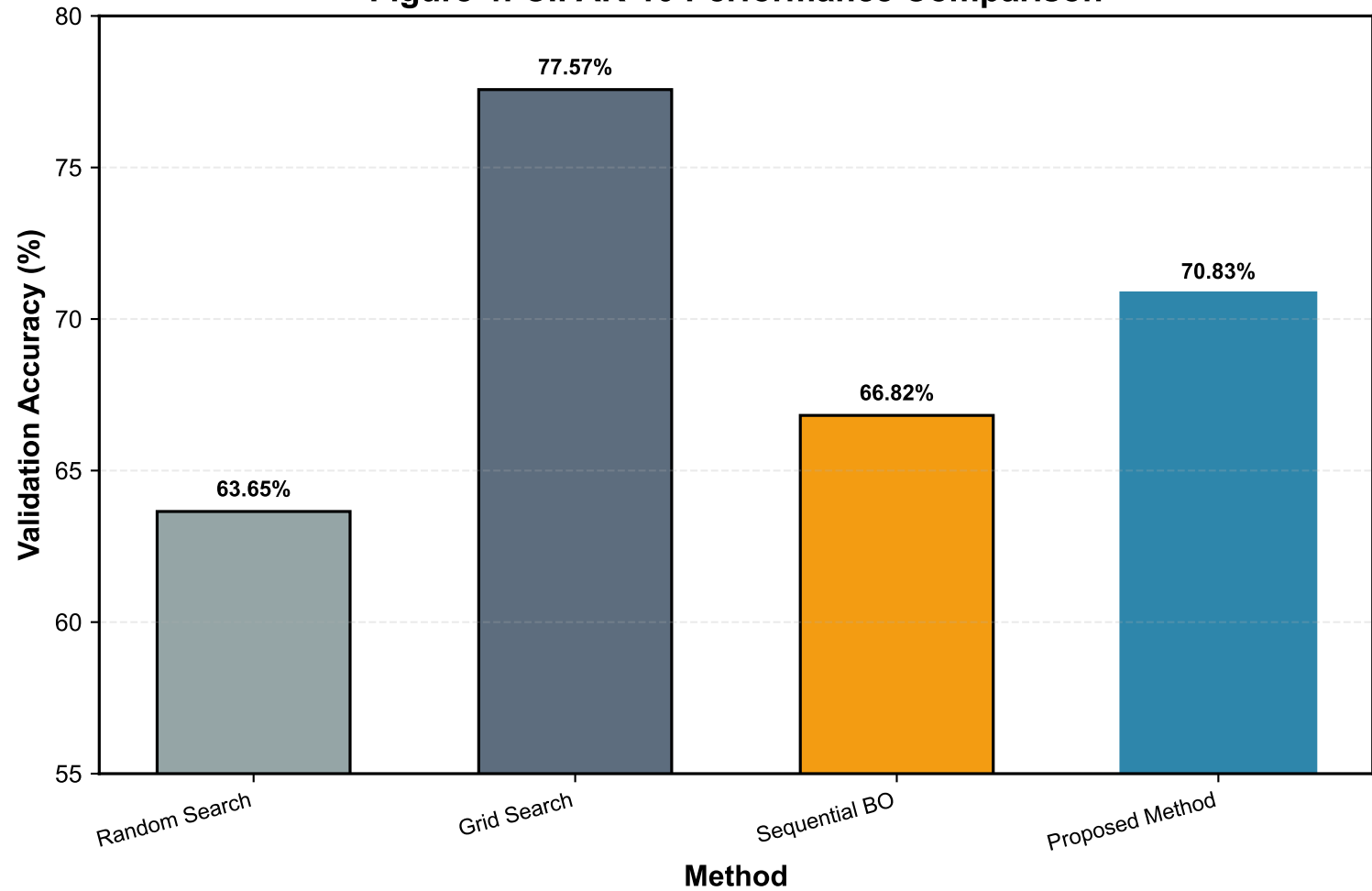
Figure 4: CIFAR-10 Performance Comparison
