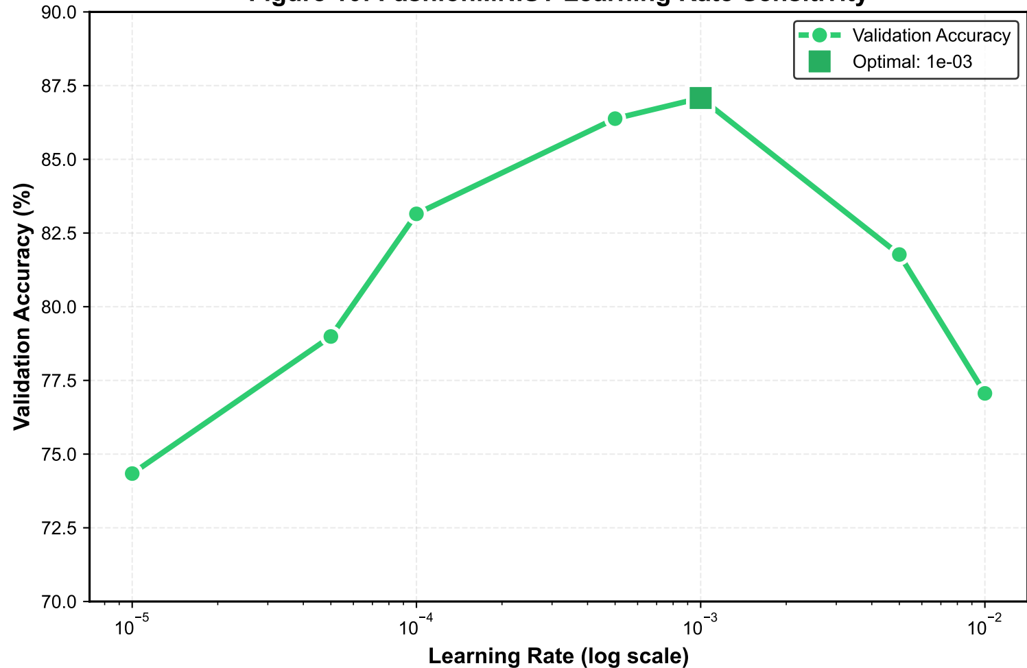
Figure 10: FashionMNIST Learning Rate Sensitivity
