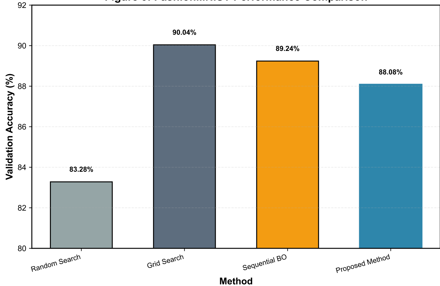
Figure 3: FashionMNIST Performance Comparison
