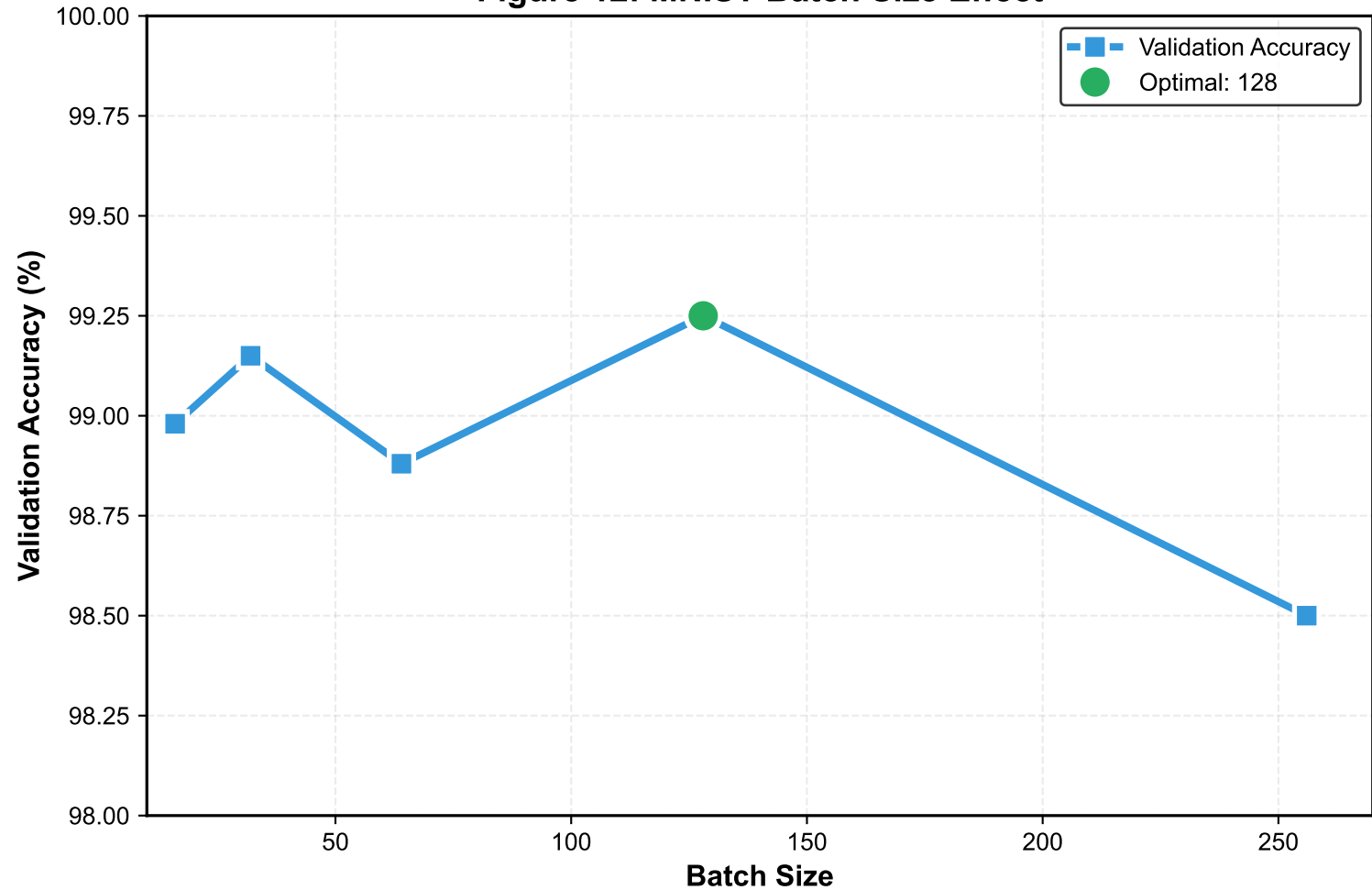
Figure 12: MNIST Batch Size Effect
