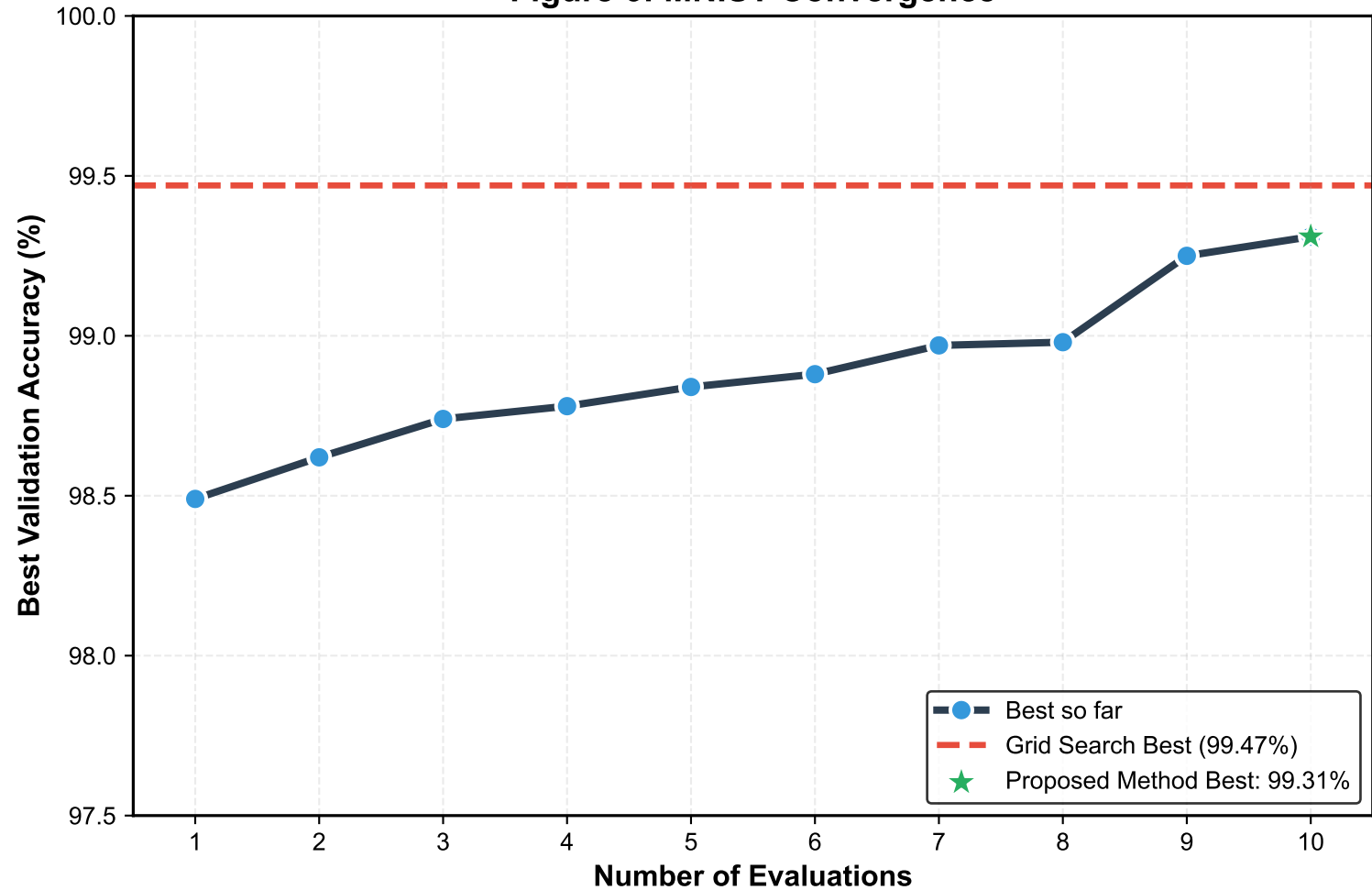
Figure 6: MNIST Convergence
