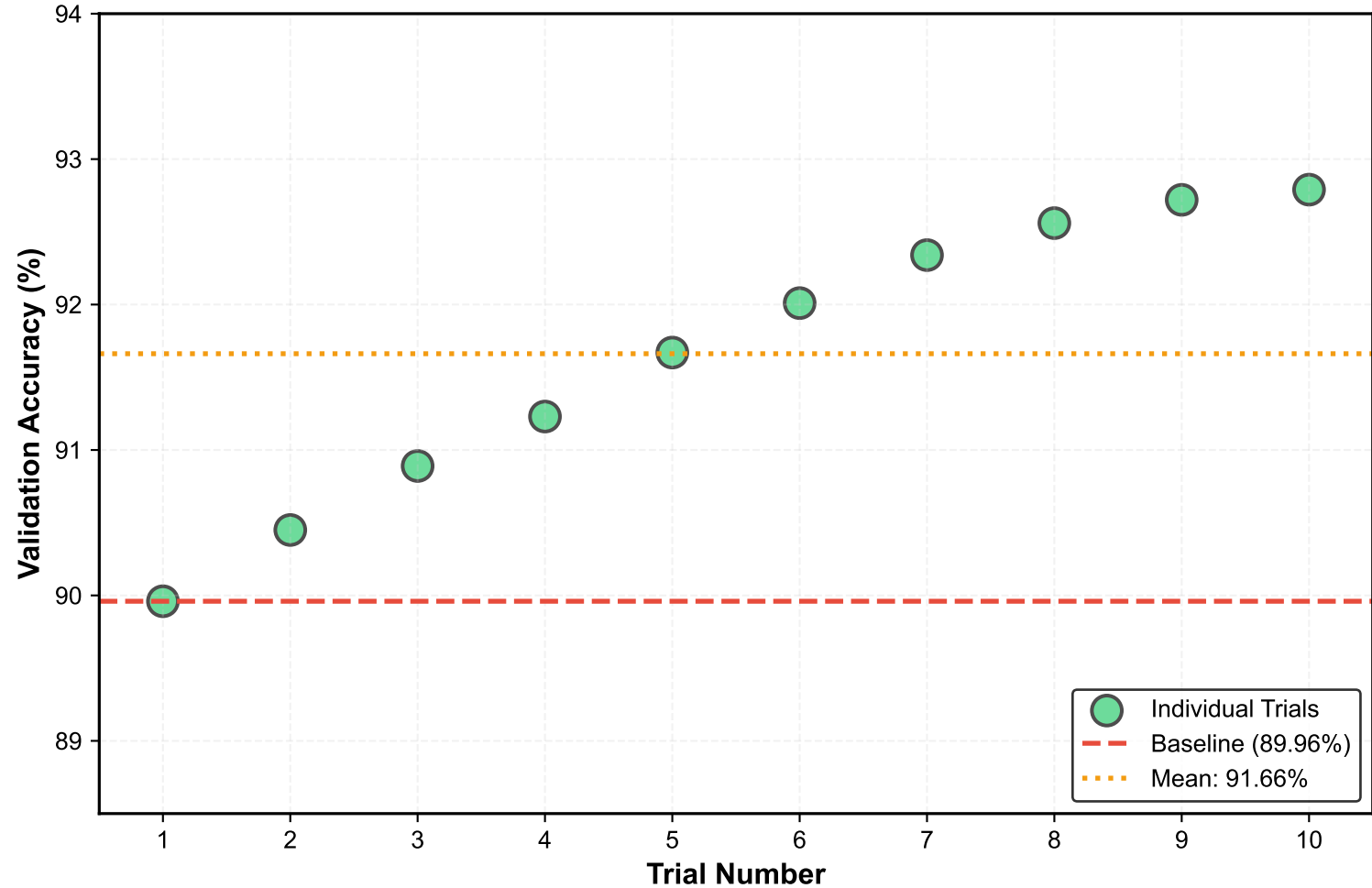
FashionMNIST: Individual Trial Performance
