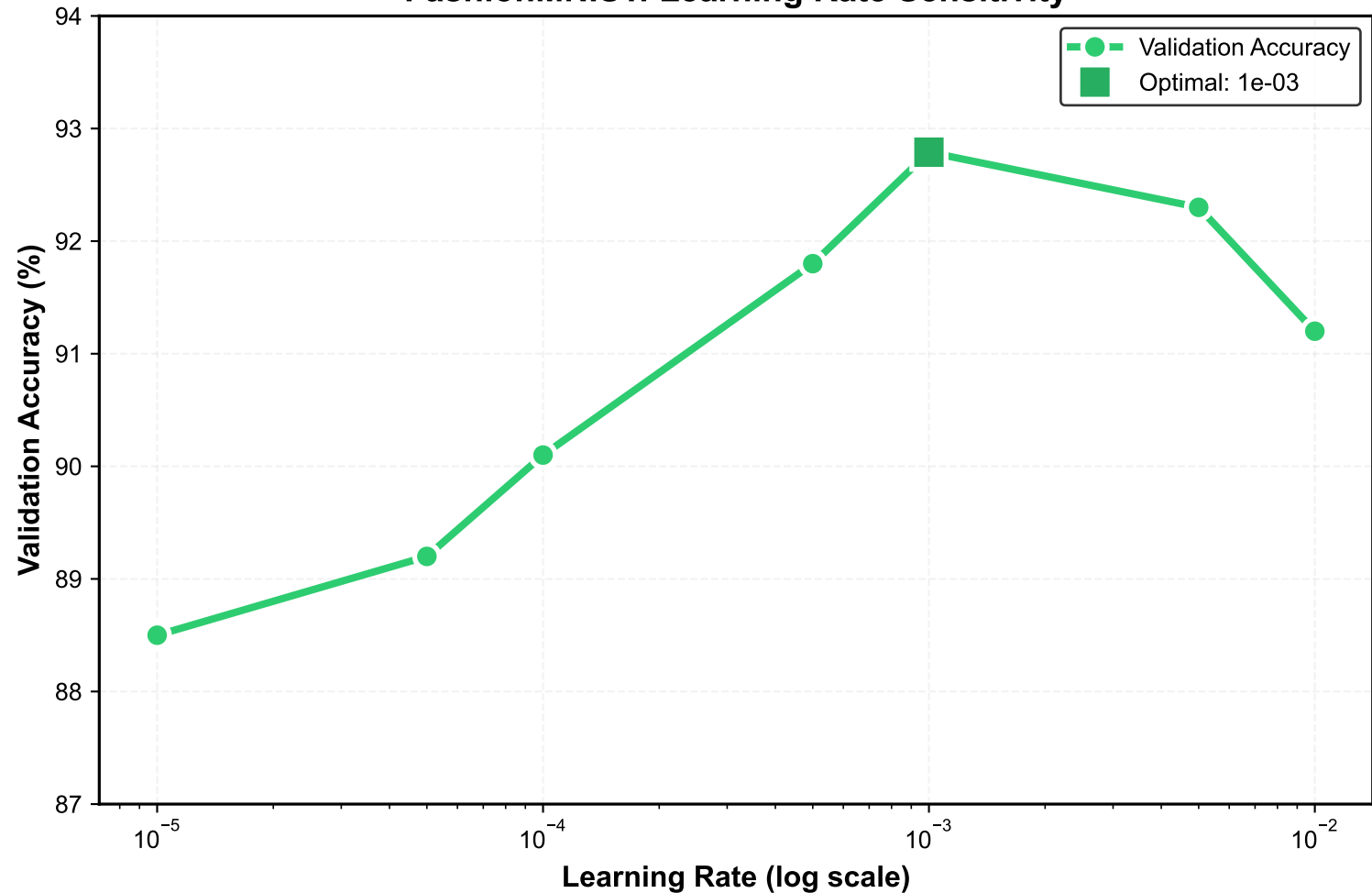
FashionMNIST: Learning Rate Sensitivity
