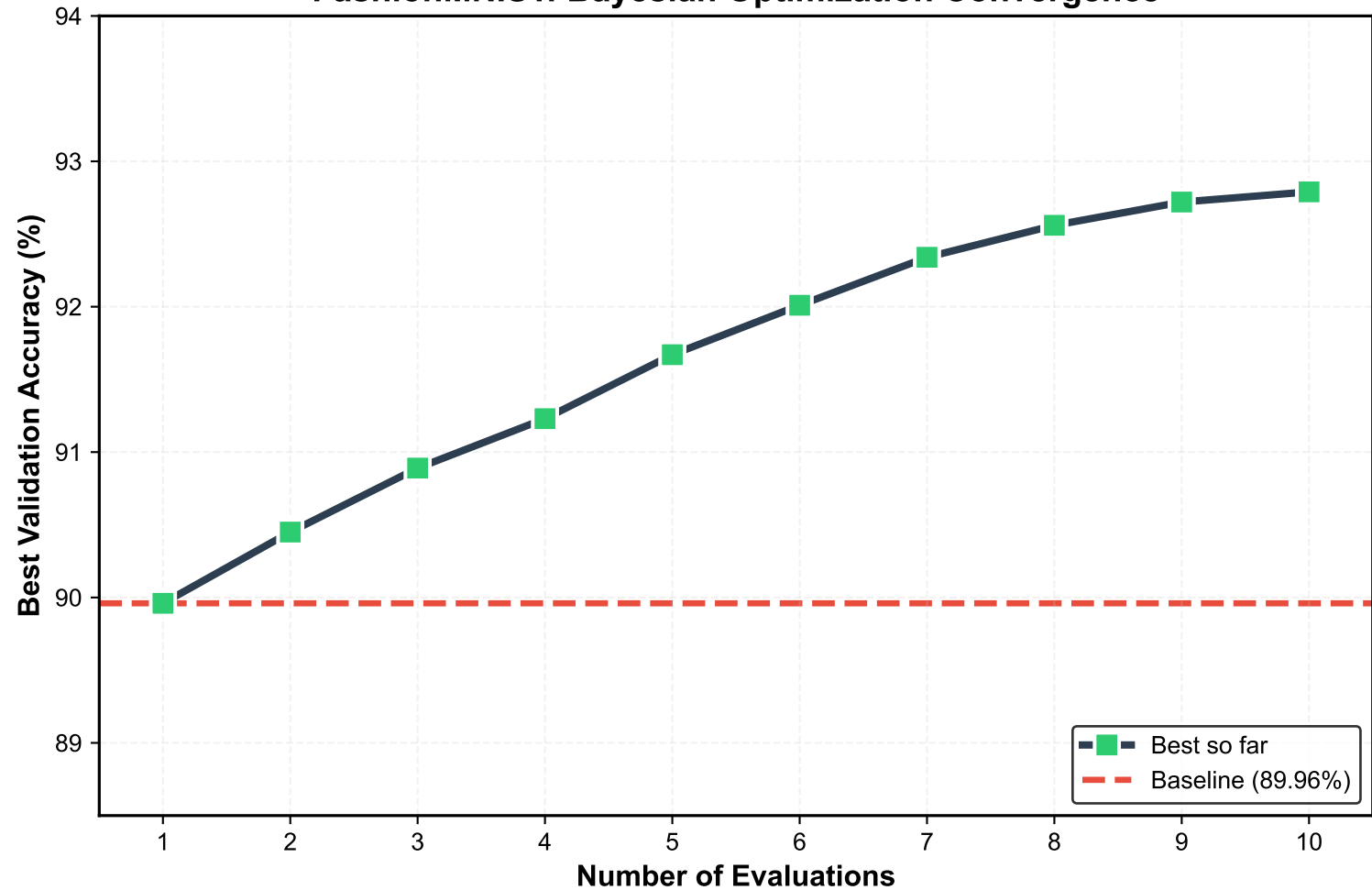
FashionMNIST: Bayesian Optimization Convergence
