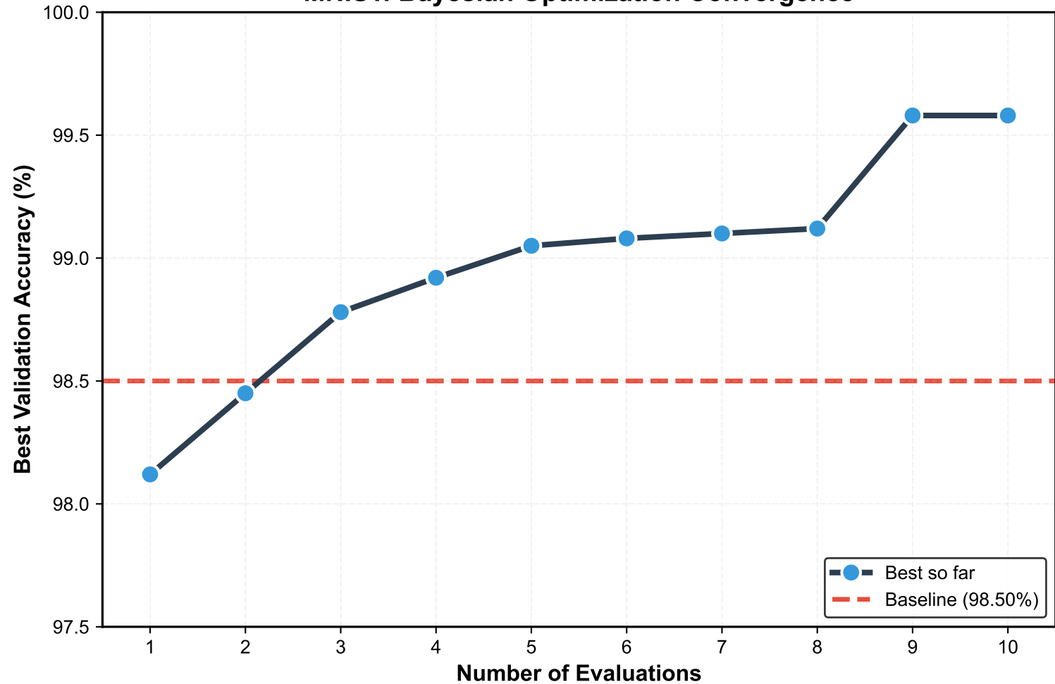
MNIST: Bayesian Optimization Convergence
