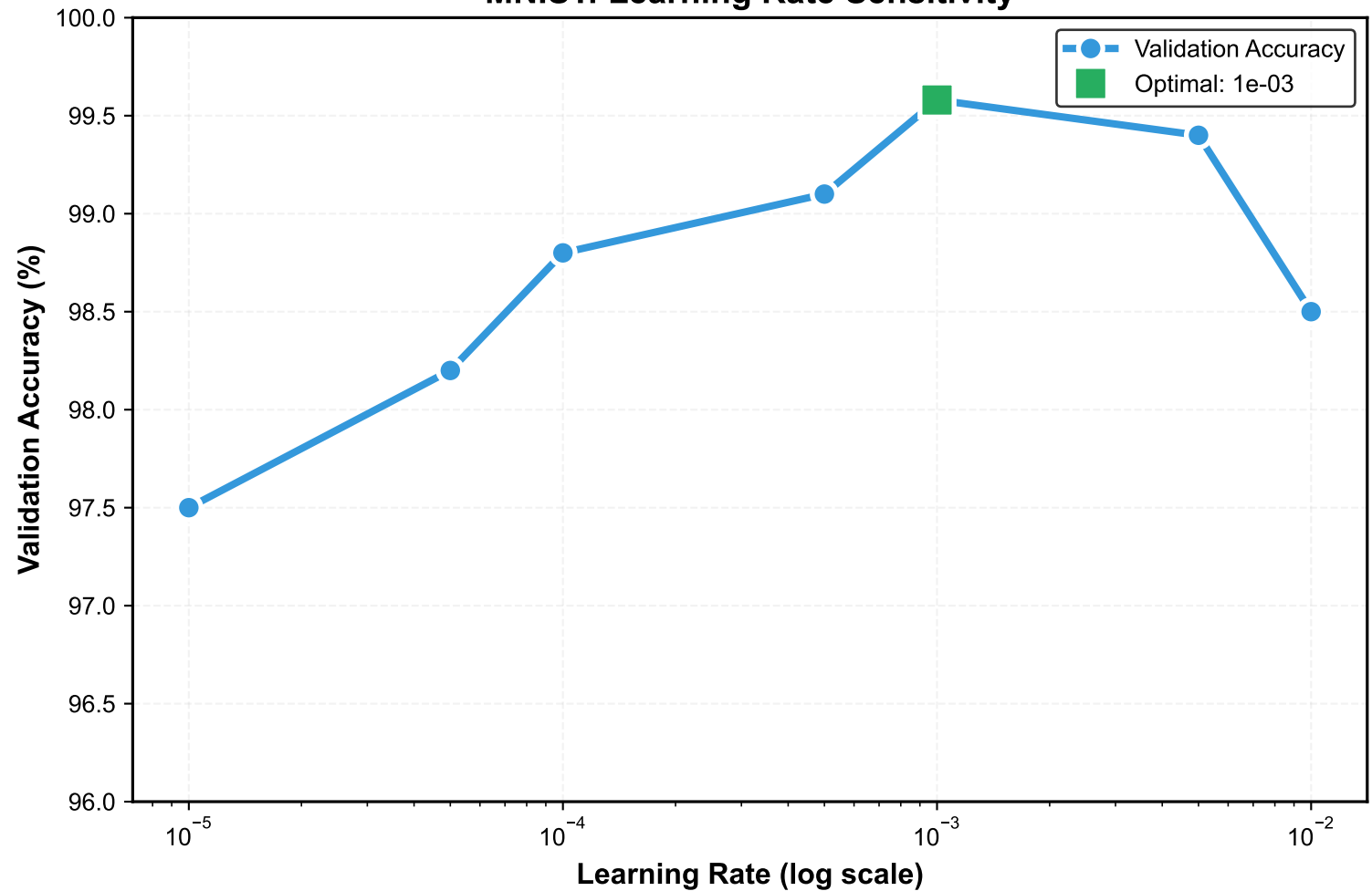
MNIST: Learning Rate Sensitivity
