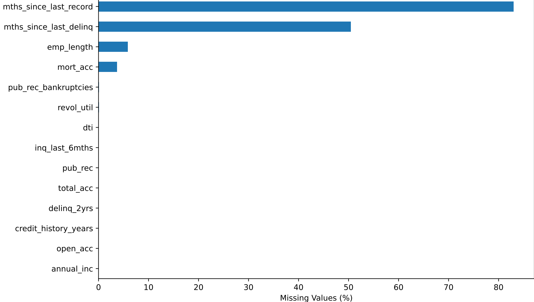
Top Features with Missing Values in Lending Club Dataset
