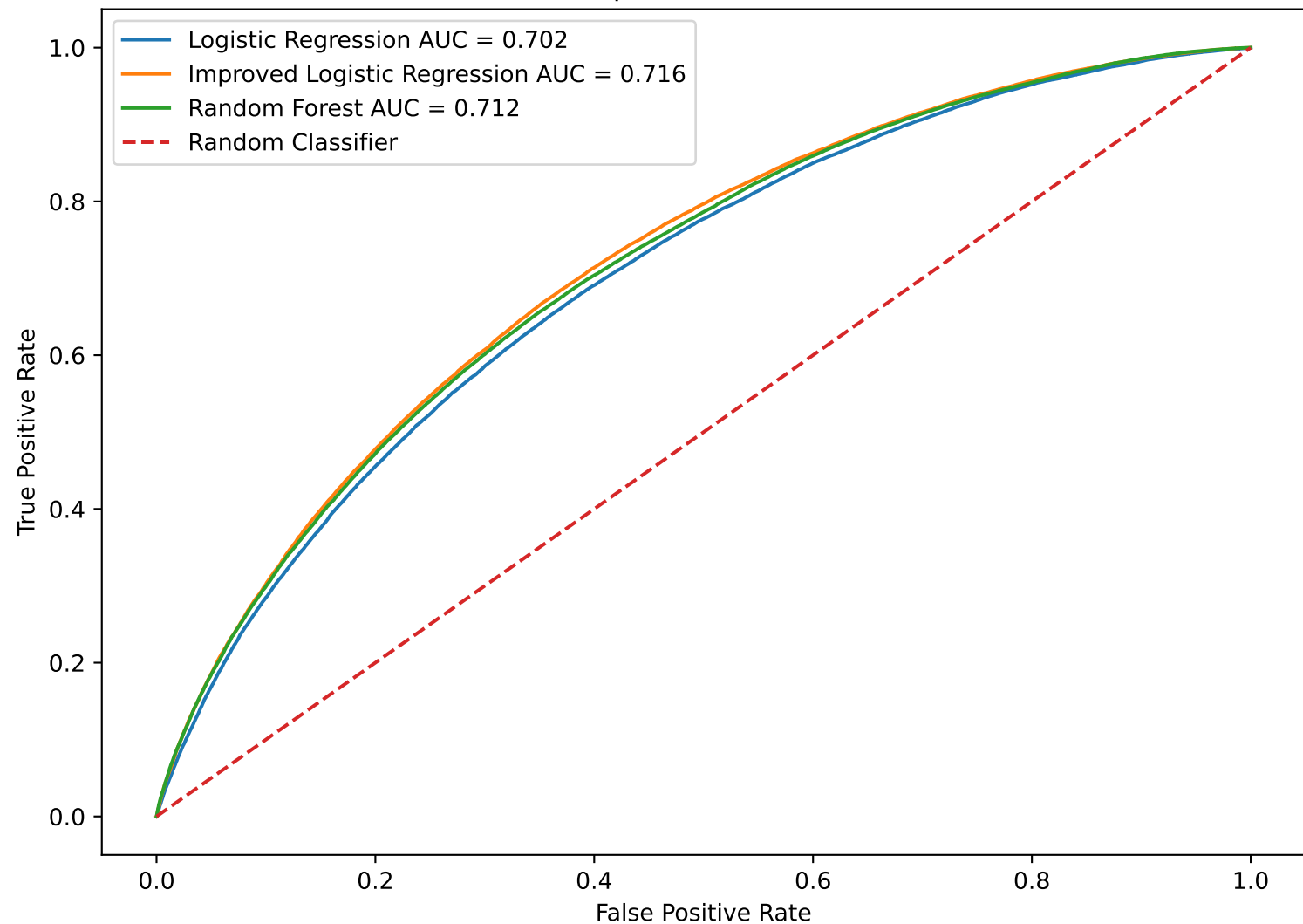
ROC Curve Comparison of Credit Risk Models
