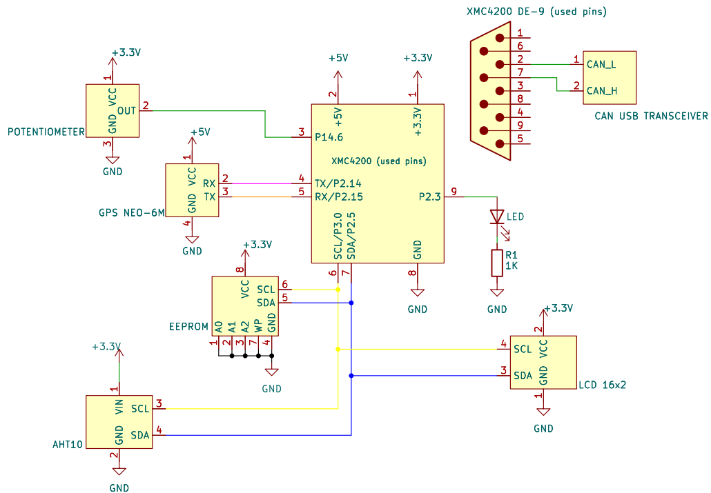
Figure 3: Electrical schematic
