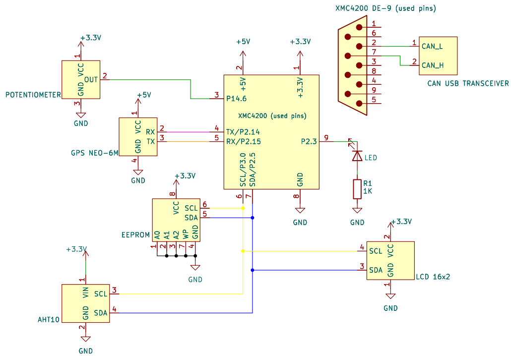
Figure 3: Electrical schematic
