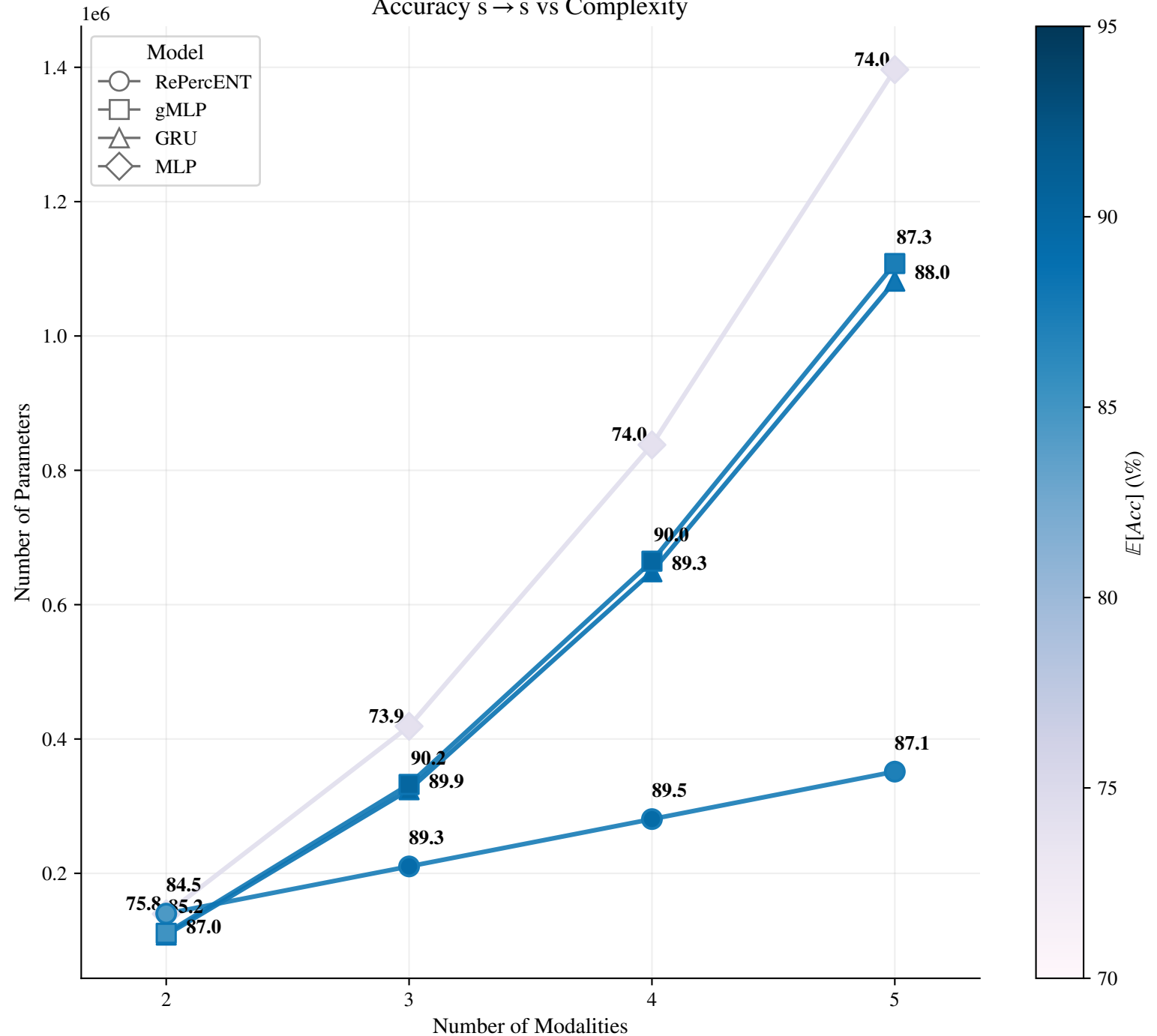
Accuracy s \rightarrow s vs Complexity
