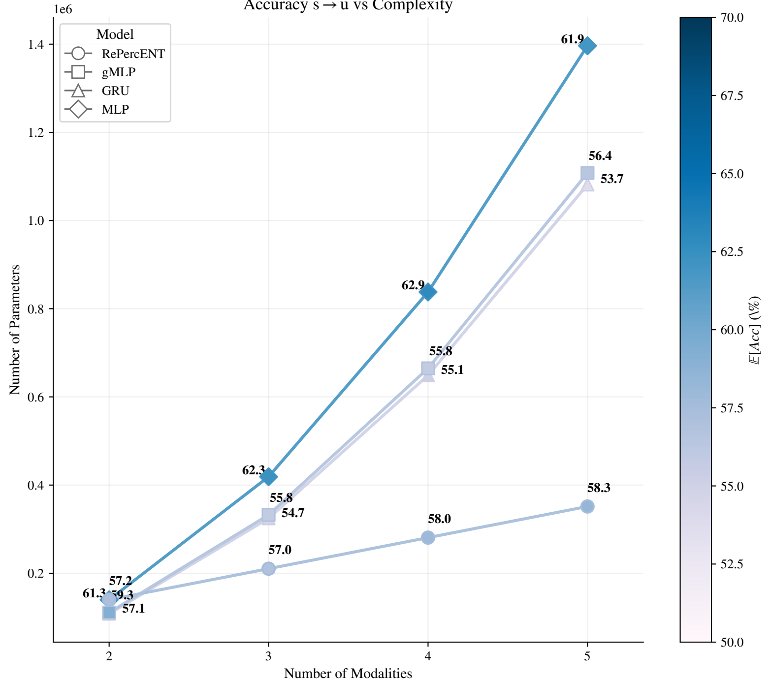
Accuracy s \rightarrow u vs Complexity
