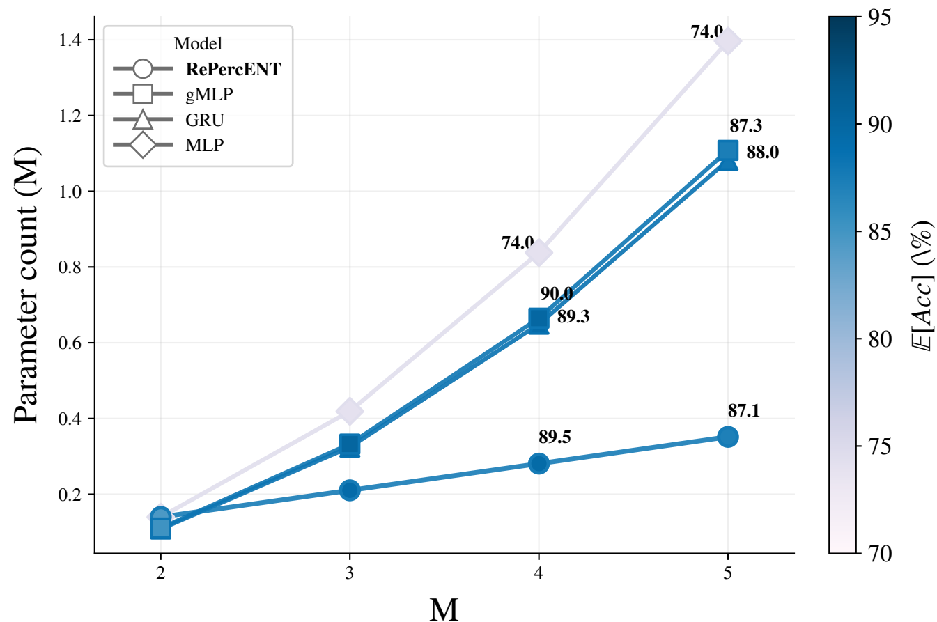
Accuracy s \rightarrow s vs Complexity
