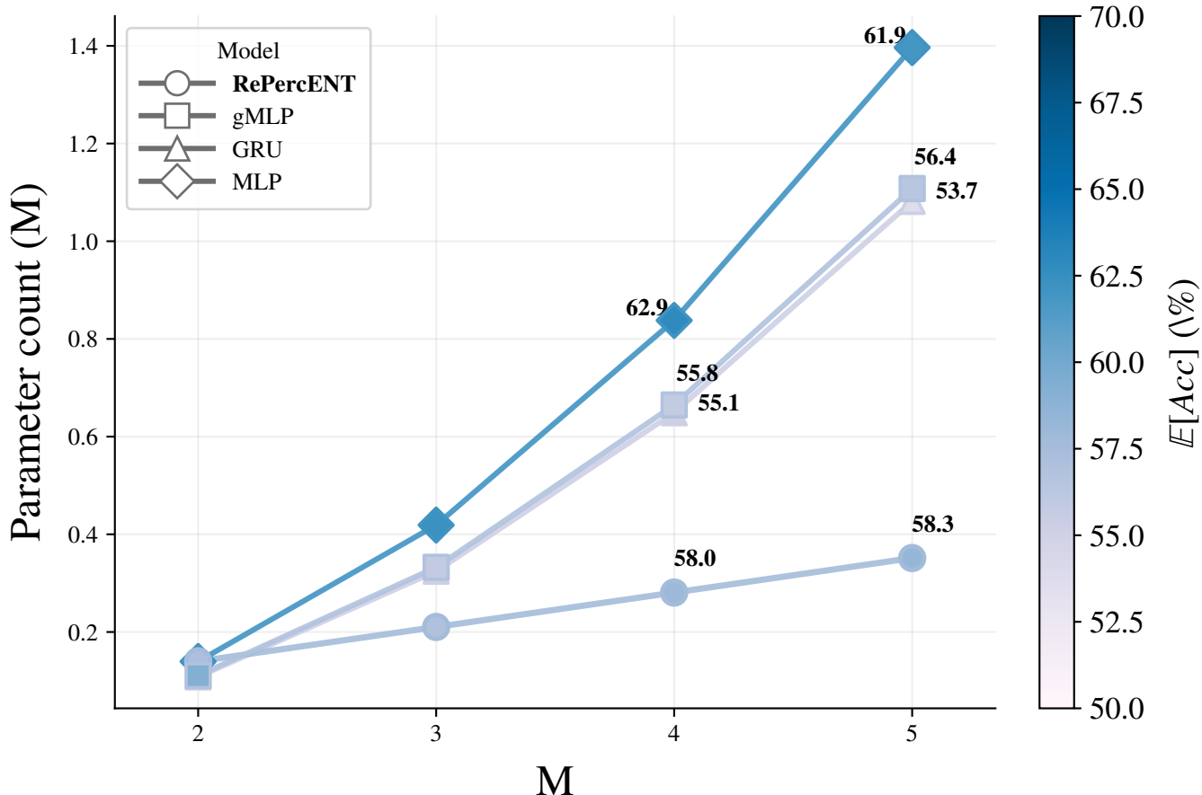
Accuracy s \rightarrow u vs Complexity
