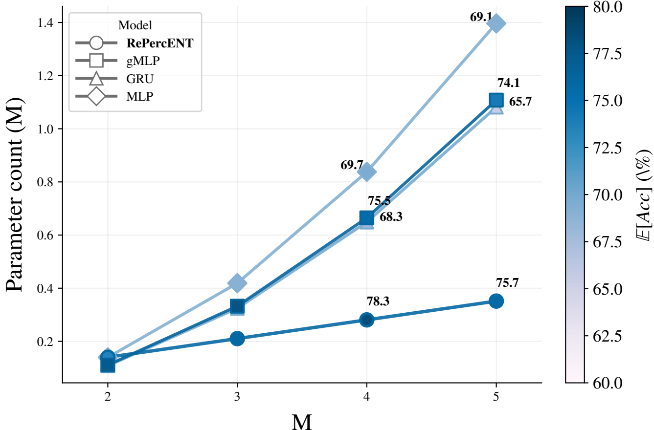
Accuracy u \rightarrow u vs Complexity
