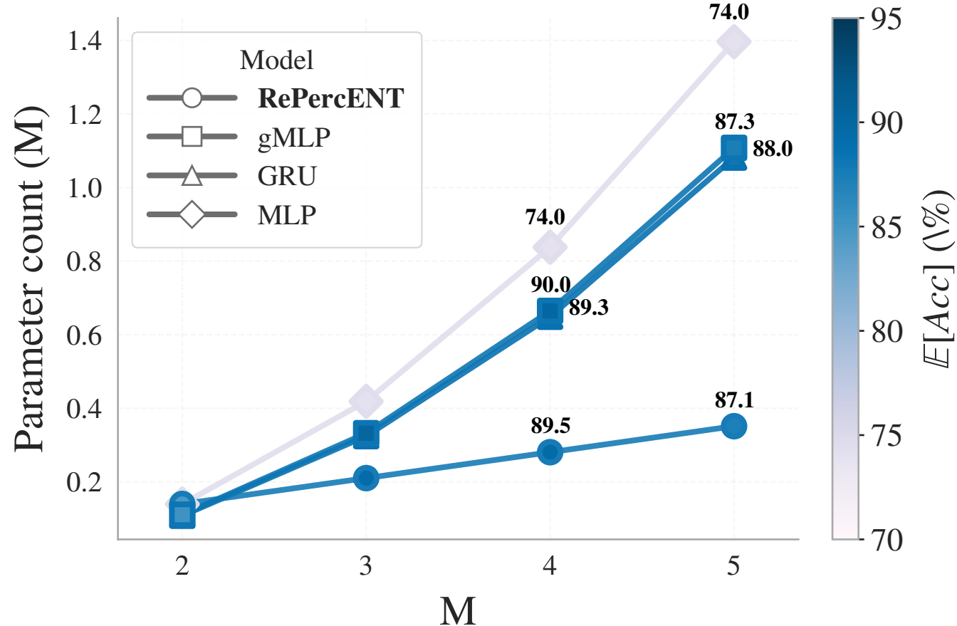
Accuracy s \rightarrow s vs Complexity
