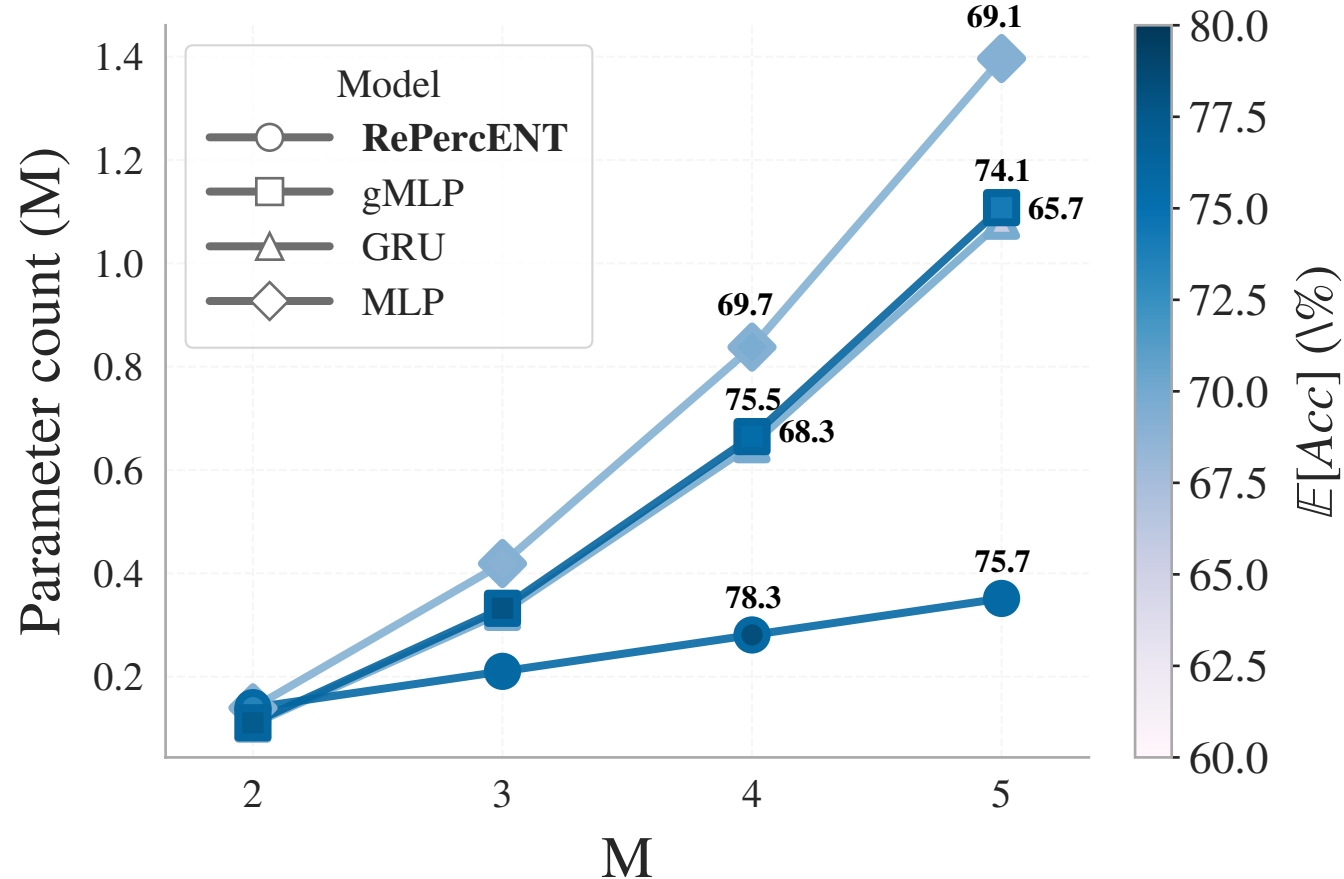
Accuracy u \rightarrow u vs Complexity
