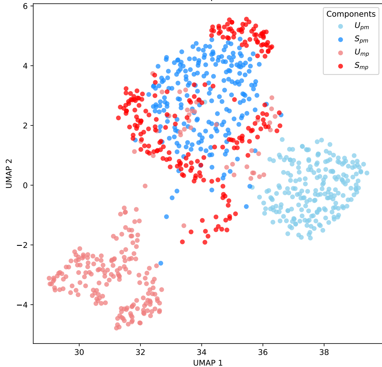
TCGA-BRCA: path vs mol
