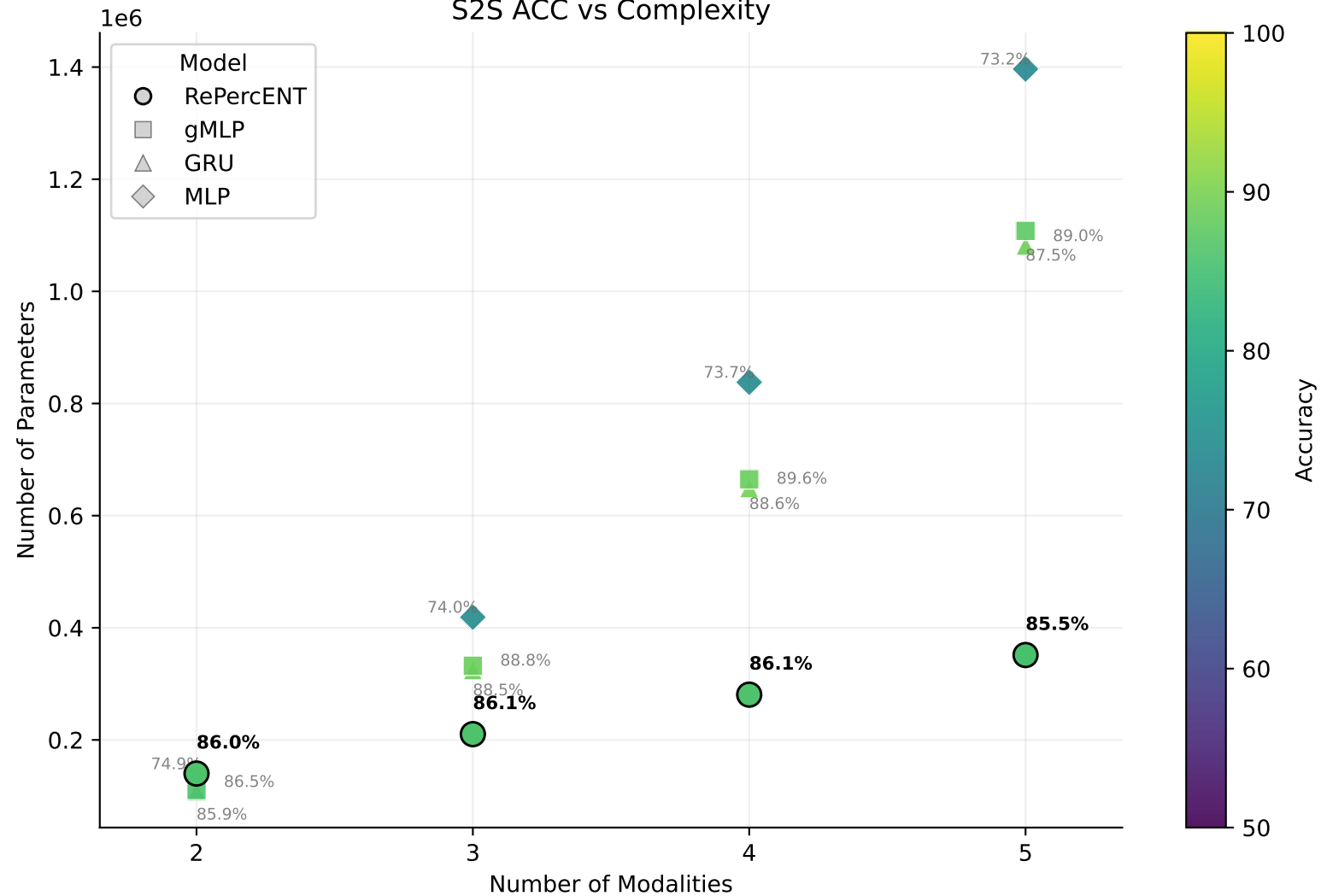
S2S ACC vs Complexity
