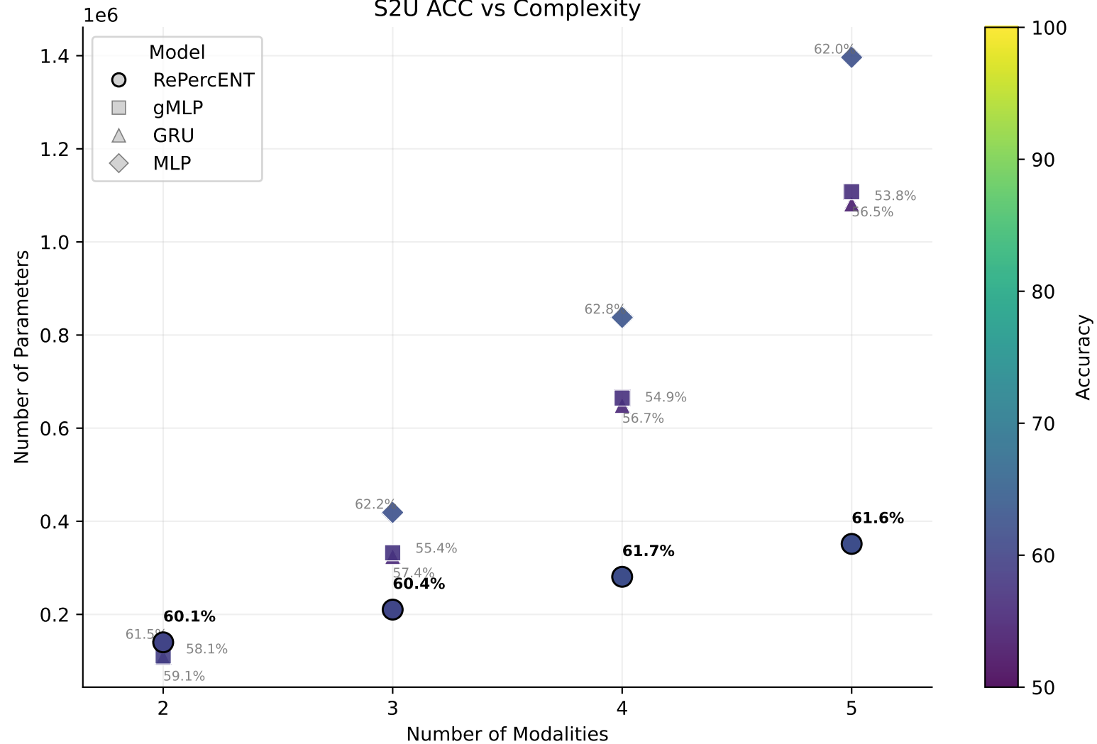
S2U ACC vs Complexity
