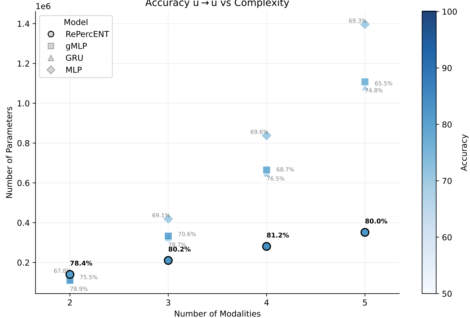
Accuracy u \rightarrow u vs Complexity
