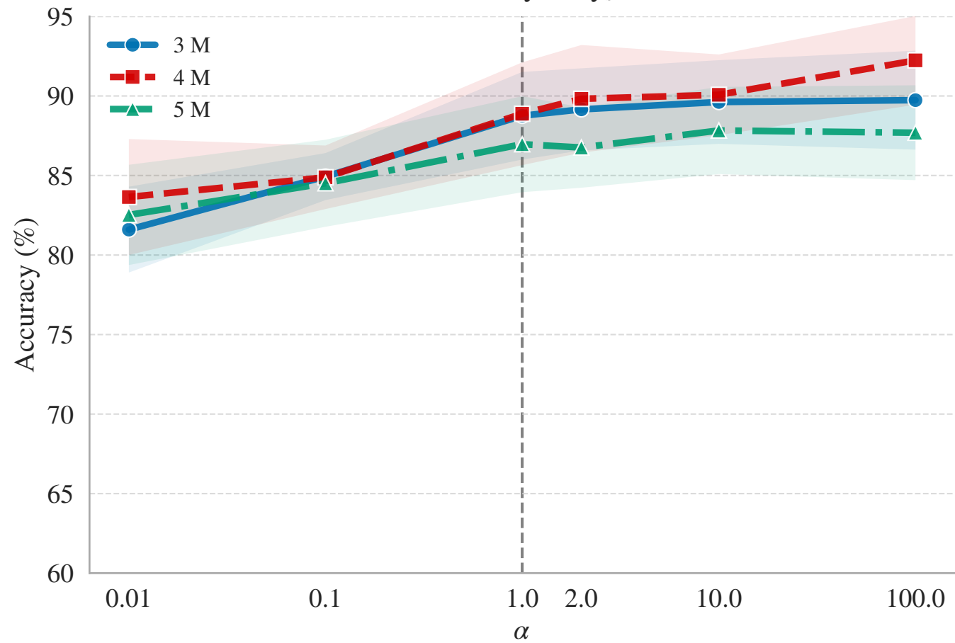
Accuracy s \rightarrow y_s
