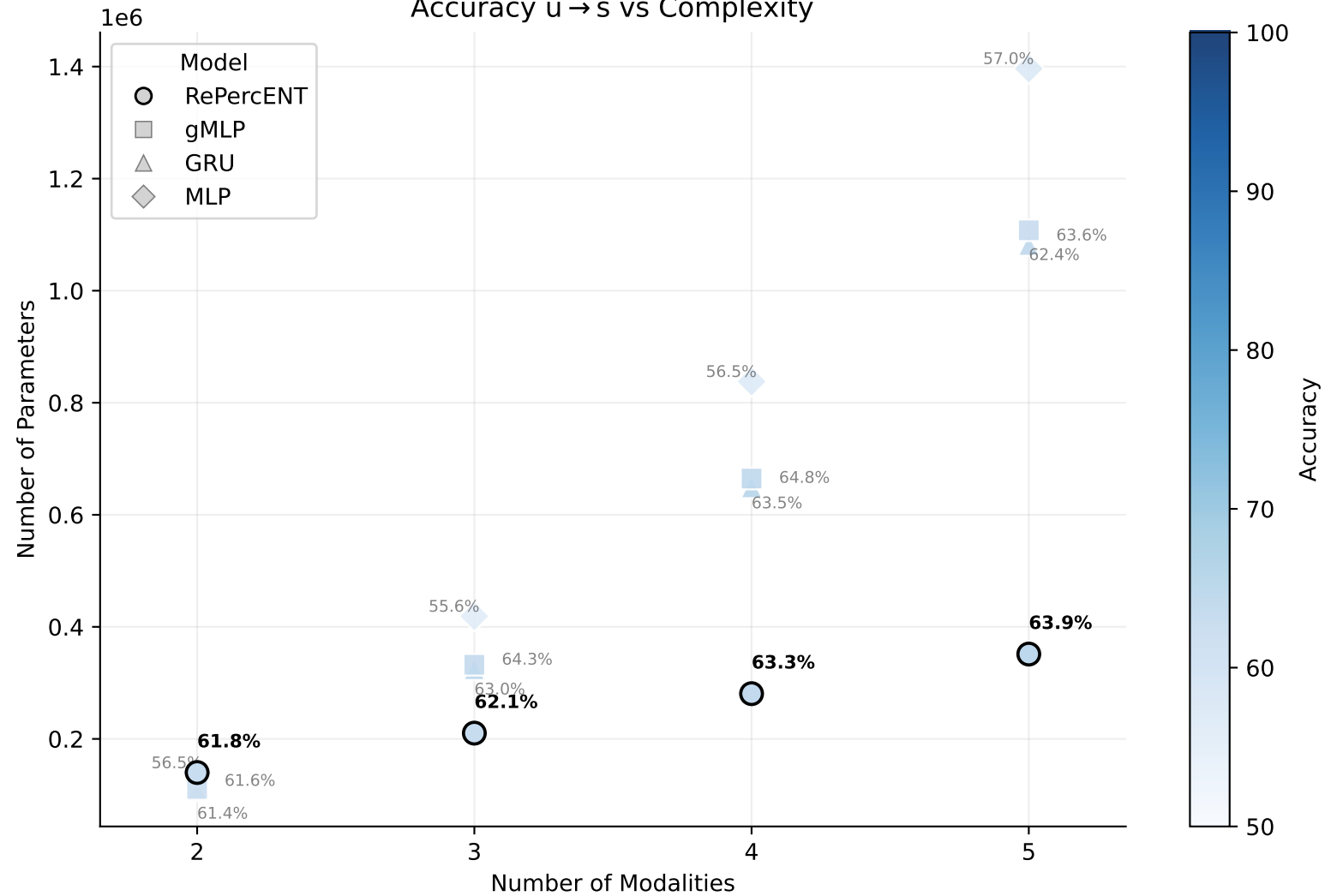
Accuracy u \rightarrow s vs Complexity
