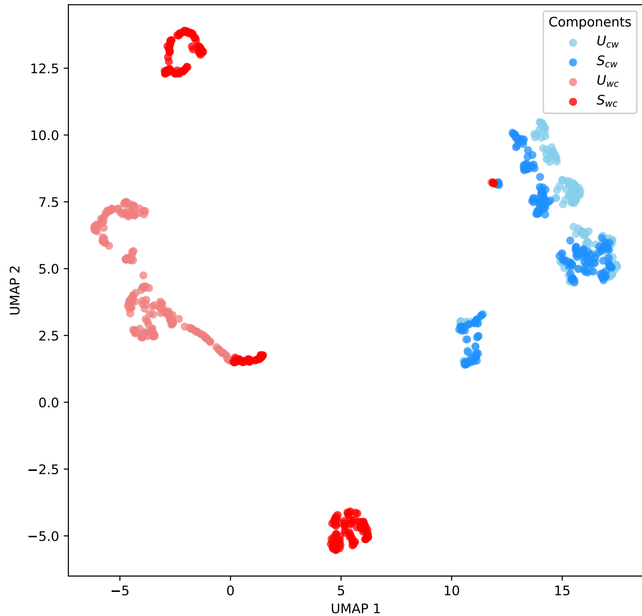
TCGA-BRCA: clin vs wsi
