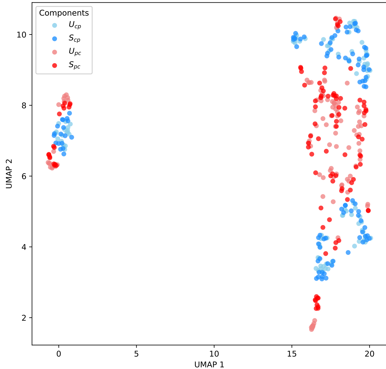
TCGA-LUSC: clin vs path
